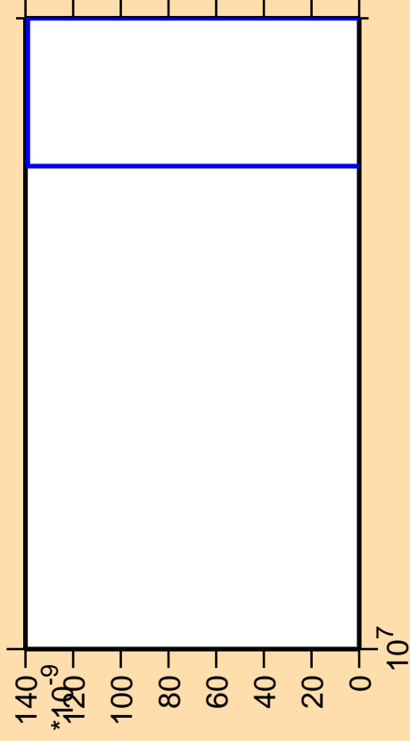
\Delta\sigma/\sigma vs. E for ^{128}\text{Sb}(\text{mt } 11)
