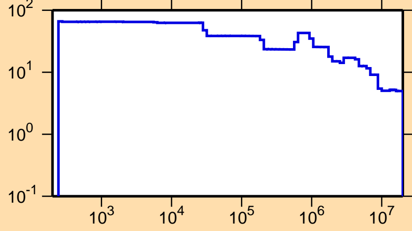
\Delta\sigma/\sigma vs. E for ^{128}\text{Sb}(n,\text{nonel.})
