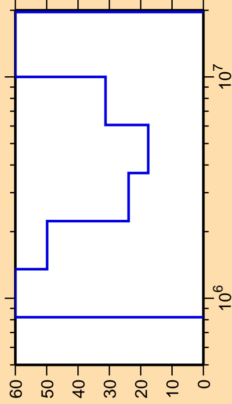
\Delta\sigma/\sigma vs. E for ^{128}\text{Sb}(n,n\text{cont.})
