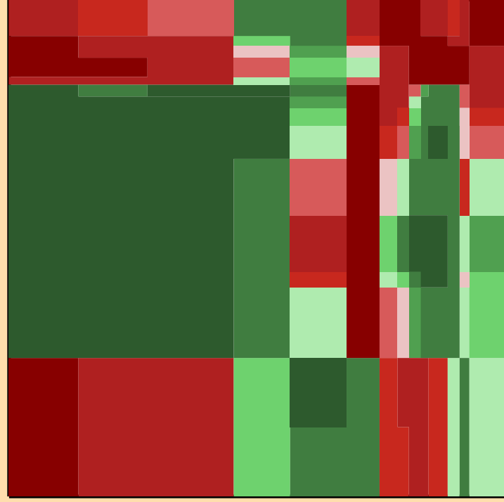
\Delta\sigma/\sigma vs. E for ^{128}\text{Sb}(n,\text{el.})
