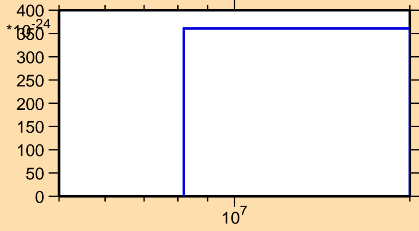
\sigma vs. E for ^{128}\text{Sb}(\text{mt } 11)
