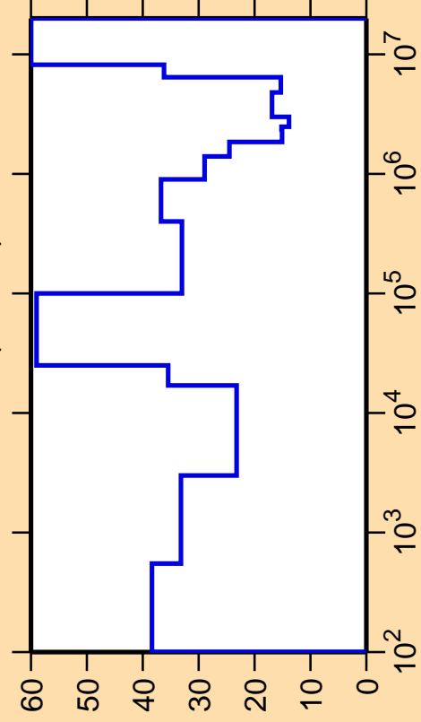
\Delta\sigma/\sigma vs. E for ^{128}\text{Sb}(n,\text{inel.})
