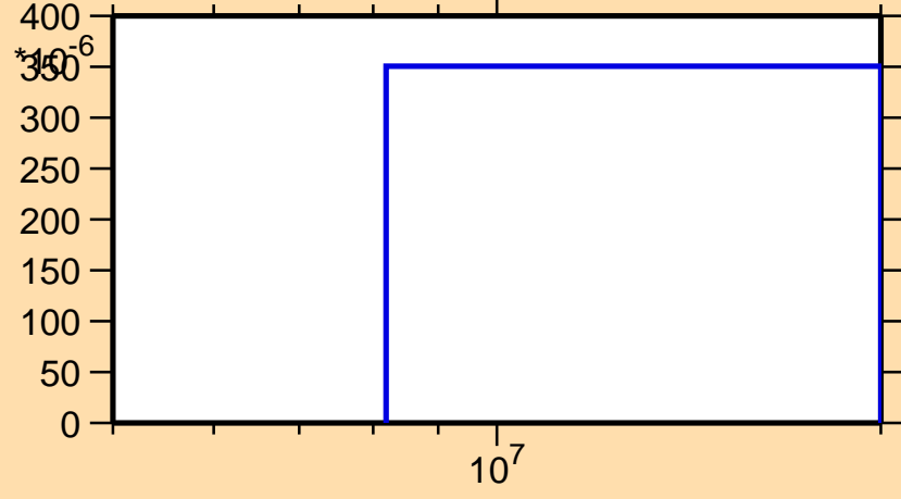
\sigma vs. E for ^{128}\text{Sb}(n,np)
