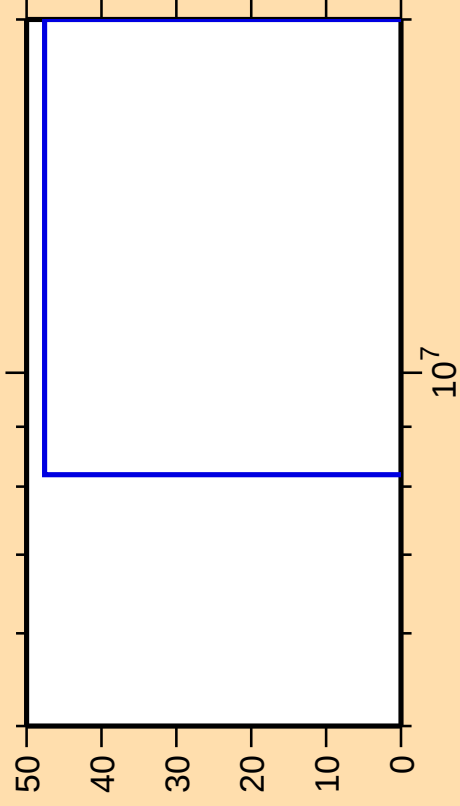
\Delta\sigma/\sigma vs. E for ^{129}\text{Sb}(n,3n)
