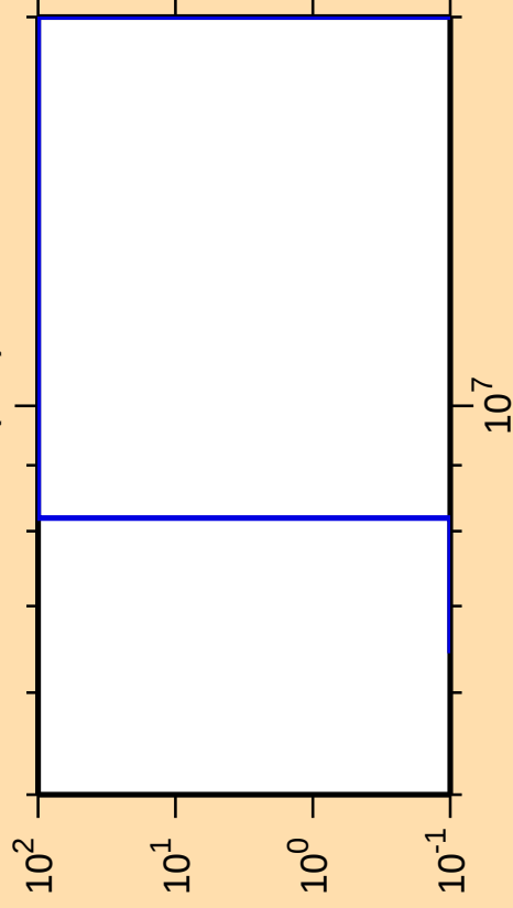
\Delta\sigma/\sigma vs. E for ^{129}\text{Sb}(n,d)
