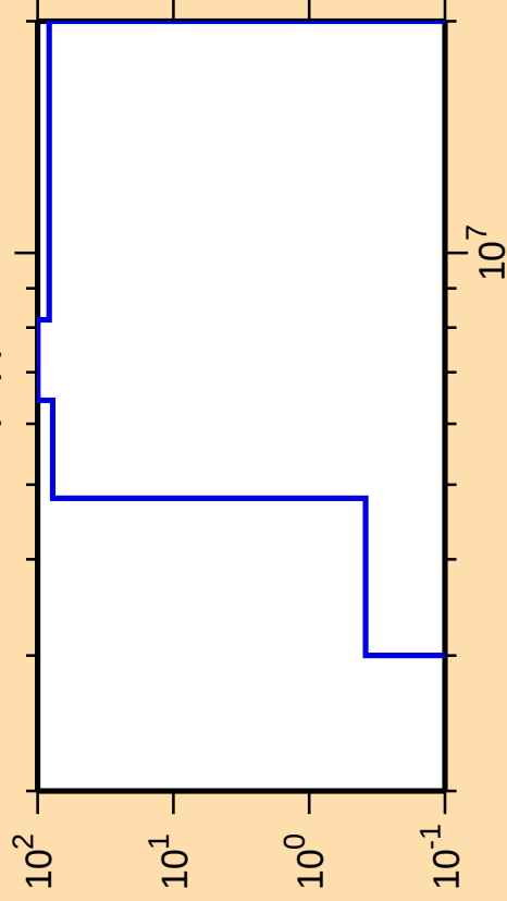
\Delta\sigma/\sigma vs. E for ^{129}\text{Sb}(n,p)
