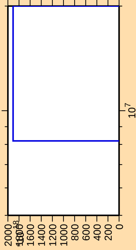
\Delta\sigma/\sigma vs. E for ^{129}\text{Sb}(\text{mt 11})
