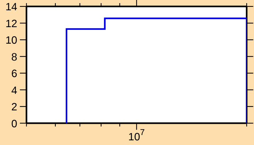
\Delta\sigma/\sigma vs. E for ^{129}\text{Sb}(n,\text{tot.})
