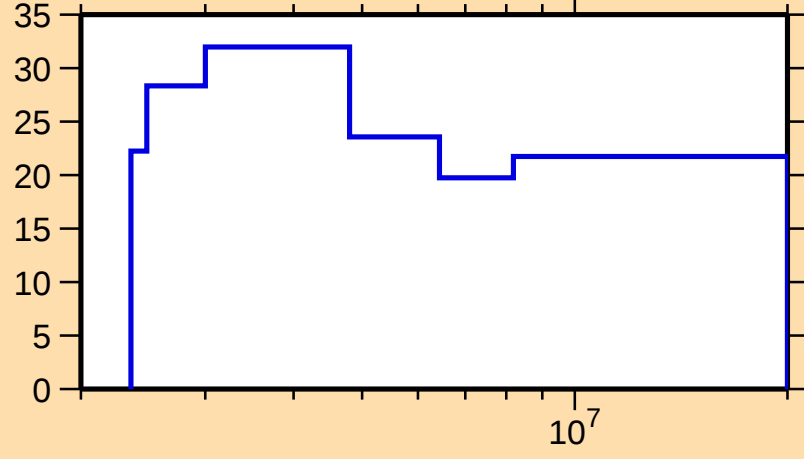
\Delta\sigma/\sigma vs. E for ^{129}\text{Sb}(n,n\text{onel.})
