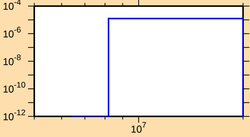
\sigma vs. E for ^{129}\text{Sb}(n,\alpha)
