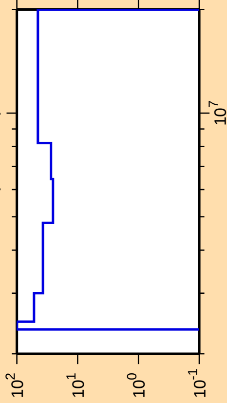
\Delta\sigma/\sigma vs. E for ^{129}\text{Sb}(n,n\text{cont.})
