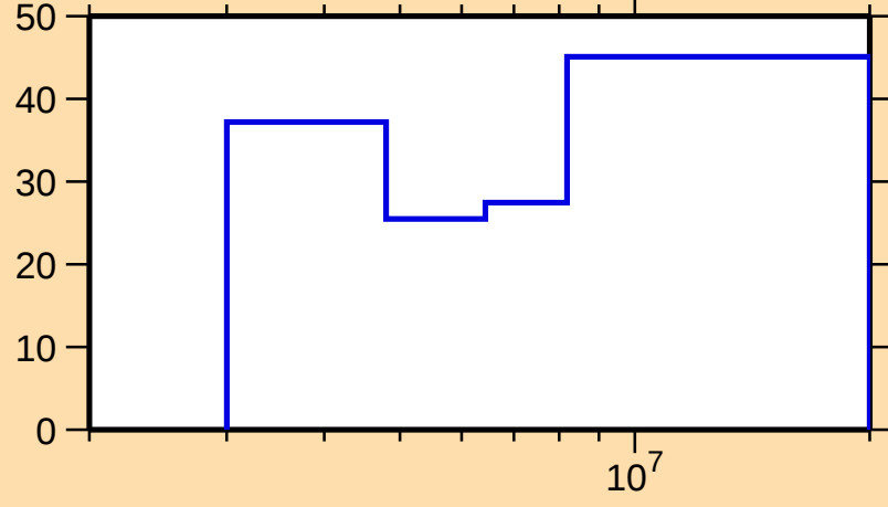
\Delta\sigma/\sigma vs. E for ^{129}\text{Sb}(n,ncont.)
