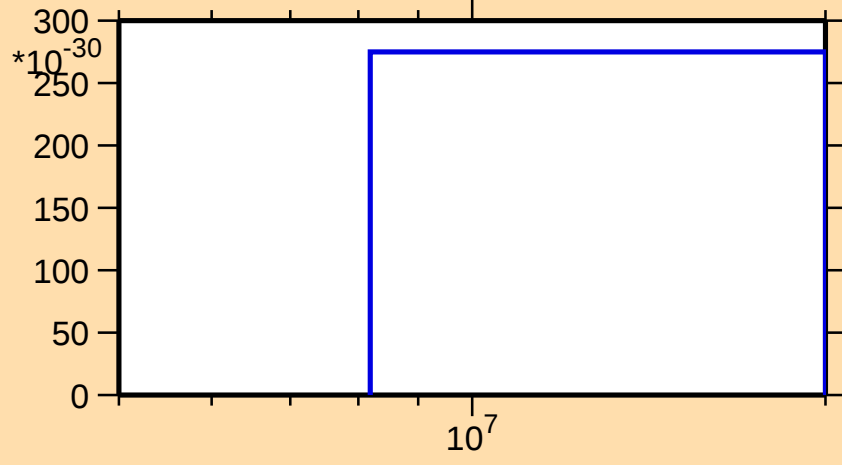
\sigma vs. E for ^{129}\text{Sb}(\text{mt 11})
