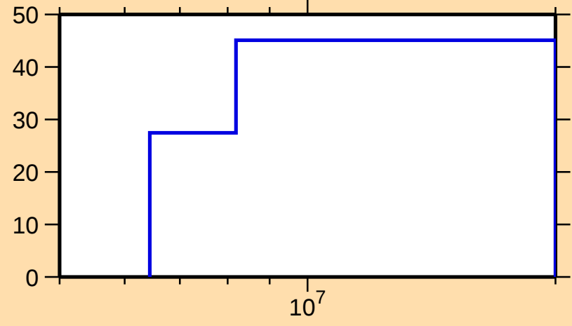
\Delta\sigma/\sigma vs. E for ^{129}\text{Sb}(n,n\text{cont.})
