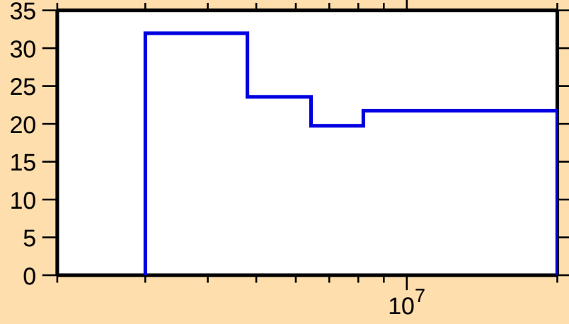
\Delta\sigma/\sigma vs. E for ^{129}\text{Sb}(n,\text{nonel.})
