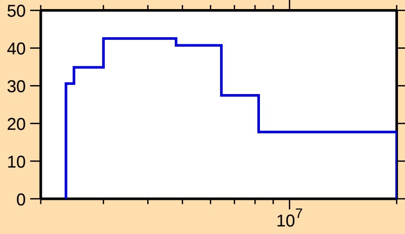
\Delta\sigma/\sigma vs. E for ^{129}\text{Sb}(n,\text{el.})
