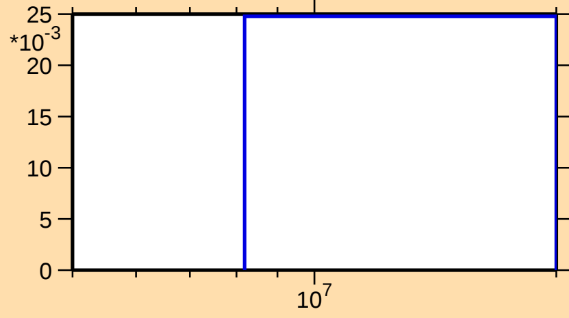
\sigma vs. E for ^{129}\text{Sb}(n,3n)
