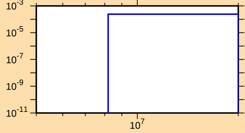
\sigma vs. E for ^{129}\text{Sb}(n,d)
