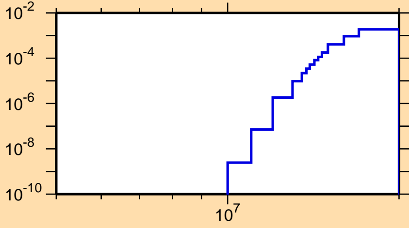
\sigma vs. E for ^{130}\text{Sb}(n,d)
