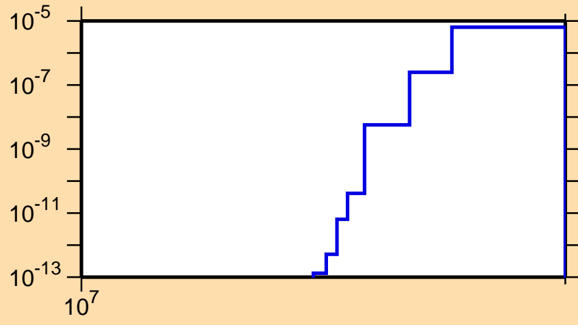
\sigma vs. E for ^{130}\text{Sb}(n,nd)
