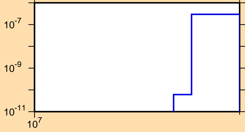
\sigma vs. E for ^{130}\text{Sb}(n,nt)
