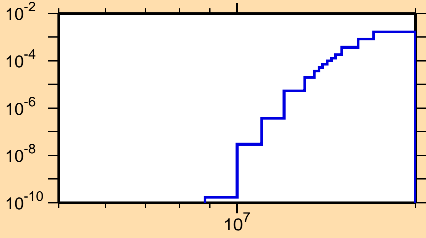
\sigma vs. E for ^{131}\text{Sb}(n,d)
