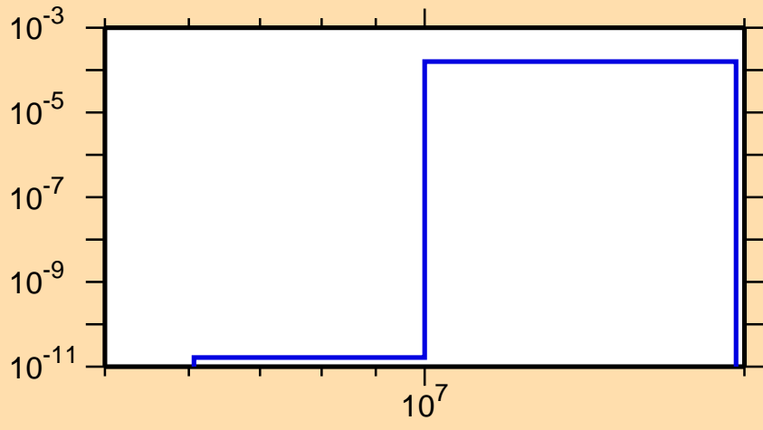
\sigma vs. E for ^{131}\text{Sb}(n,d)
