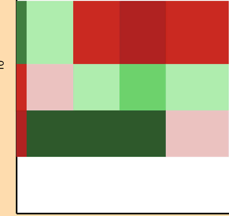
Correlation Matrix
