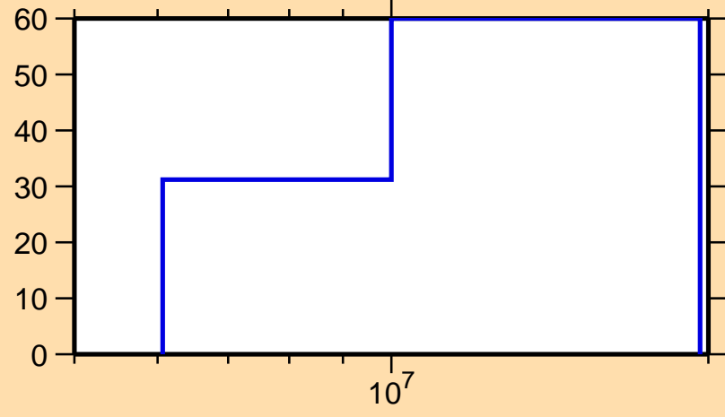
\Delta\sigma/\sigma vs. E for ^{131}\text{Sb}(n,n\text{cont.})
