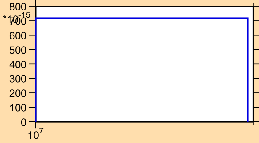
\sigma vs. E for ^{131}\text{Sb}(n,2np)
