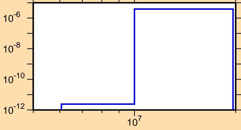
\sigma vs. E for ^{131}\text{Sb}(n,\alpha)
