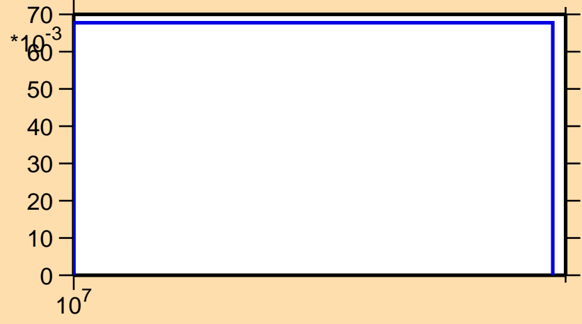
\sigma vs. E for ^{131}\text{Sb}(n,3n)
