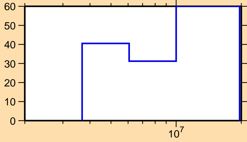
\Delta\sigma/\sigma vs. E for ^{131}\text{Sb}(n,ncont.)
