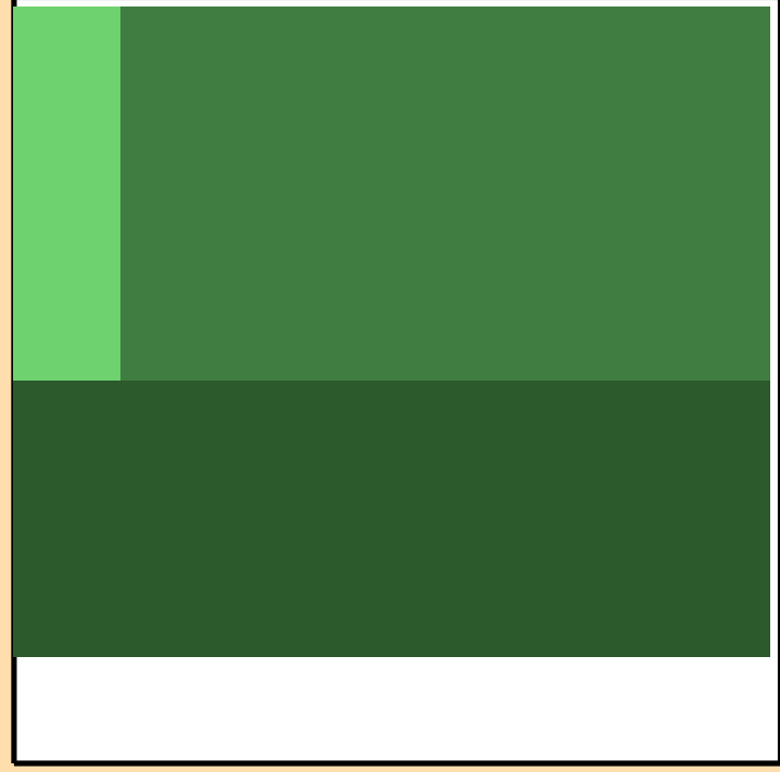
\Delta\sigma/\sigma vs. E for ^{131}\text{Sb}(n,n_1)
