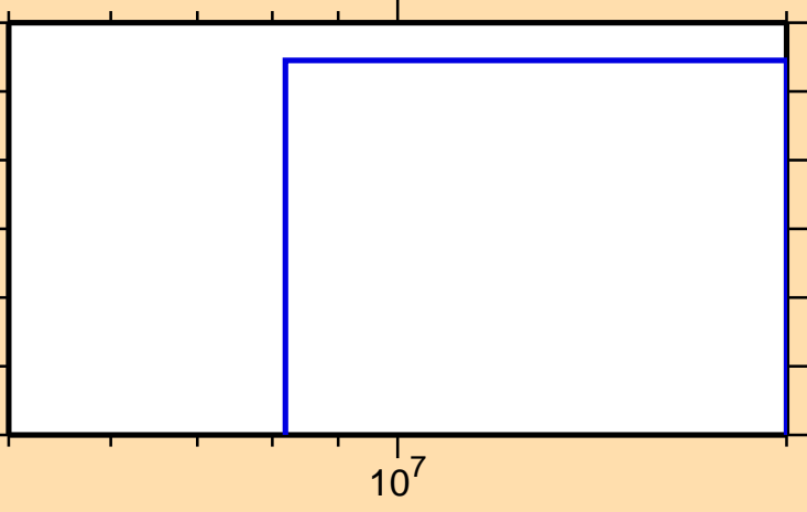
\sigma vs. E for ^{131}\text{Sb}(n,3n)
