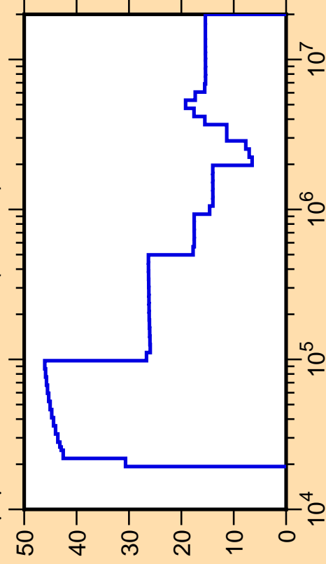
\Delta\mu/\mu vs. E for ^{132}\text{Sb}(\text{mt251})
