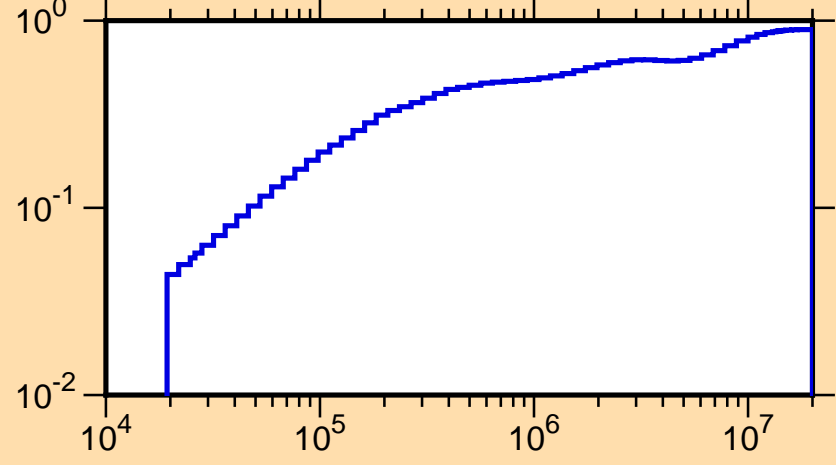
\mu vs. E for ^{132}\text{Sb}(\text{mt251})
