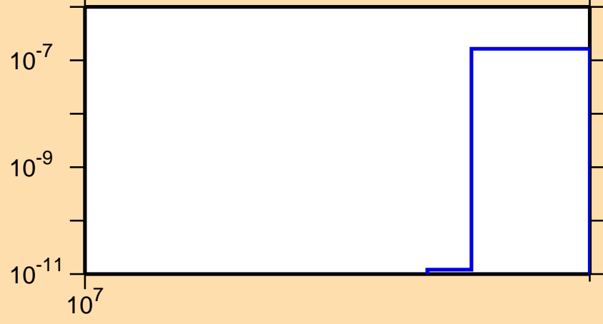
\sigma vs. E for ^{132}\text{Sb}(n,nt)
