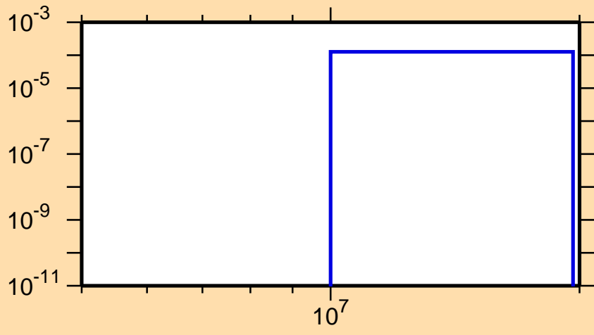
\sigma vs. E for ^{132}\text{Sb}(n,d)
