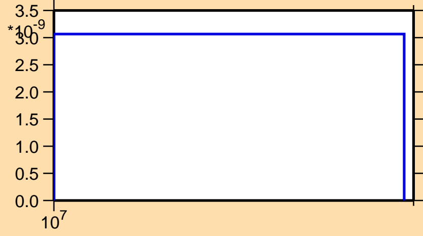
\sigma vs. E for ^{132}\text{Sb}(n,n\alpha)
