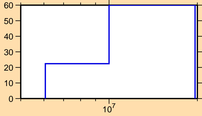
\Delta\sigma/\sigma vs. E for ^{132}\text{Sb}(n,ncont.)
