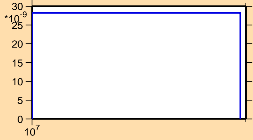
\sigma vs. E for ^{132}\text{Sb}(n,nd)
