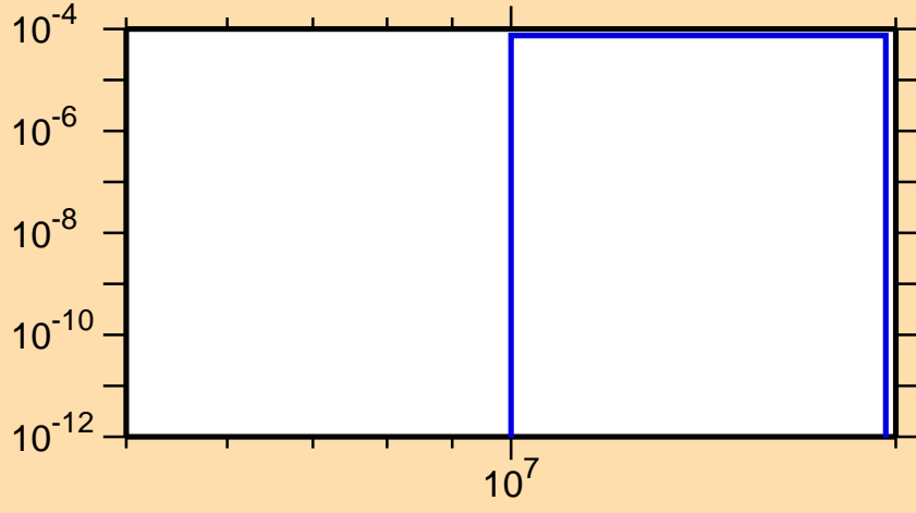
\sigma vs. E for ^{132}\text{Sb}(n,np)
