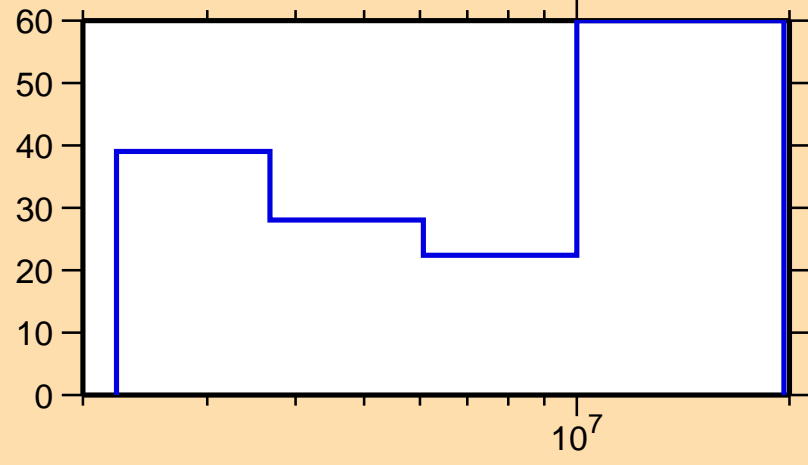
\Delta\sigma/\sigma vs. E for ^{132}\text{Sb}(n,n\text{cont.})
