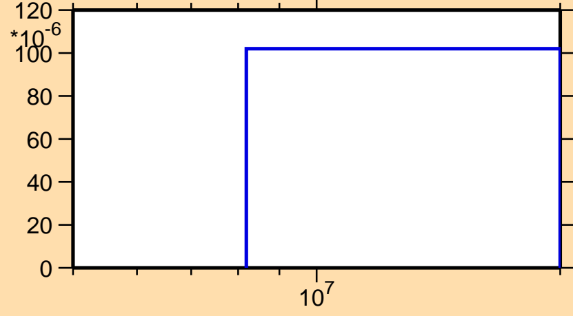
\sigma vs. E for ^{132}\text{Sb}(n,d)
