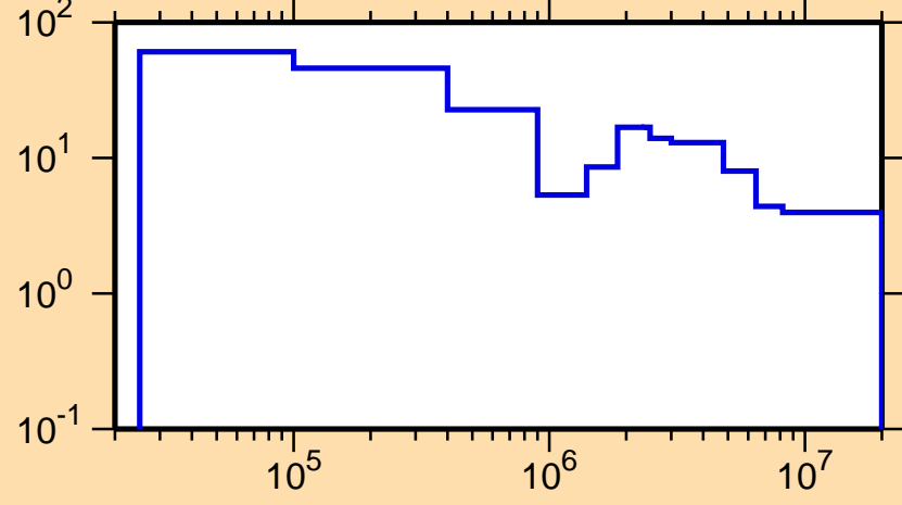
\Delta\sigma/\sigma vs. E for ^{132}\text{Sb}(n,\text{tot.})
