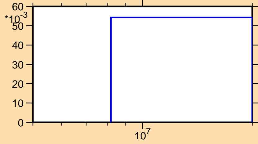
\sigma vs. E for ^{132}\text{Sb}(n,3n)
