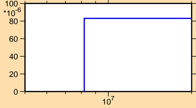
\sigma vs. E for ^{132}\text{Sb}(n,np)
