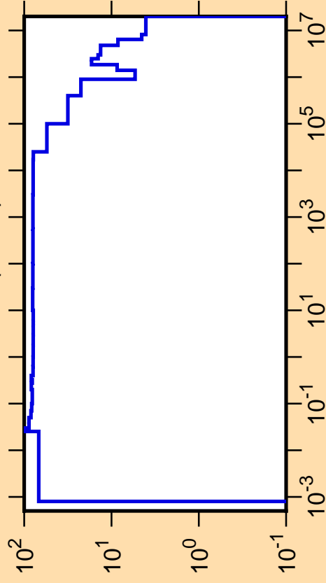
\Delta\sigma/\sigma vs. E for ^{132}\text{Sb}(n,\text{tot.})
