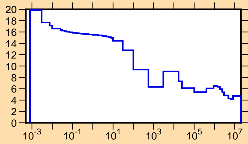
\sigma vs. E for ^{132}\text{Sb}(n,\text{tot.})
