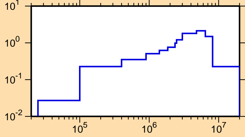
\sigma vs. E for ^{132}\text{Sb}(n,\text{inel.})
