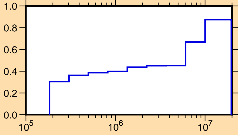
\mu vs. E for ^{133}\text{Sb}(\text{mt251})
