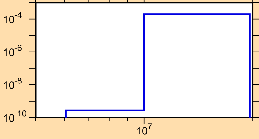
\sigma vs. E for ^{133}\text{Sb}(n,p)
