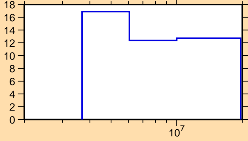
\Delta\sigma/\sigma vs. E for ^{133}\text{Sb}(n,n\text{nonel.})
