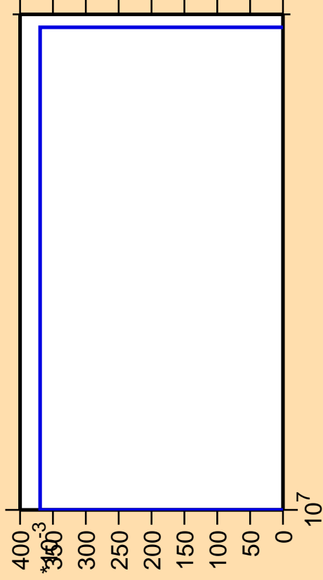
\Delta\sigma/\sigma vs. E for ^{133}\text{Sb}(n,2np)
