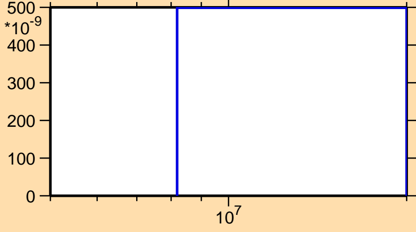
\sigma vs. E for ^{133}\text{Sb}(n,\alpha)
