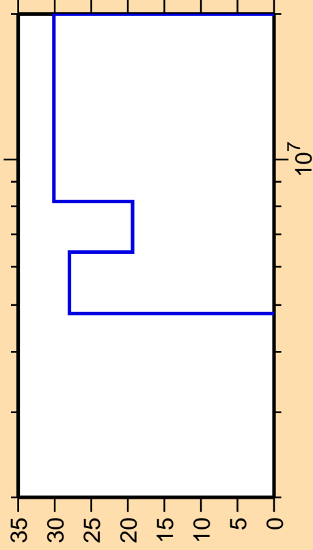
\Delta\sigma/\sigma vs. E for ^{133}\text{Sb}(n,n\text{cont.})
