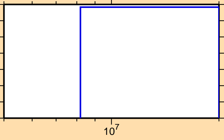
\sigma vs. E for ^{133}\text{Sb}(n,n\alpha)
