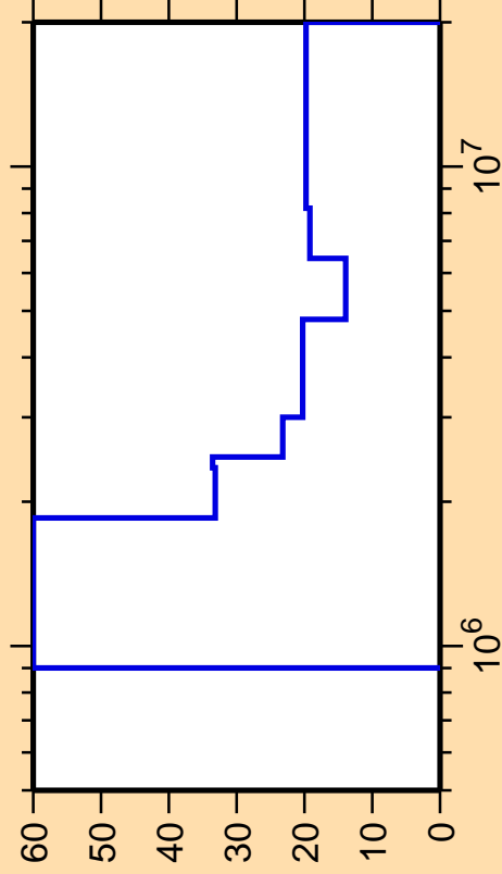
\Delta\sigma/\sigma vs. E for ^{133}\text{Sb}(n,\text{inel.})
