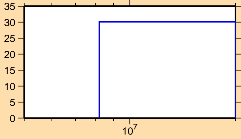
\Delta\sigma/\sigma vs. E for ^{133}\text{Sb}(n,n\text{cont.})
