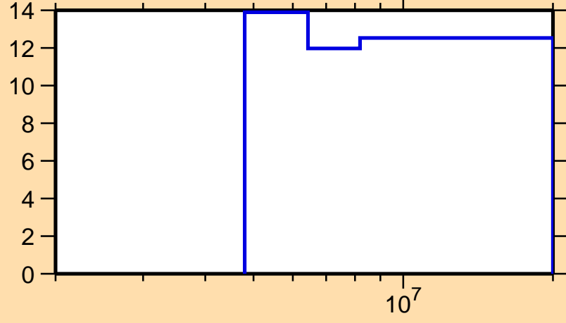
\Delta\sigma/\sigma vs. E for ^{133}\text{Sb}(n,n\text{onel.})
