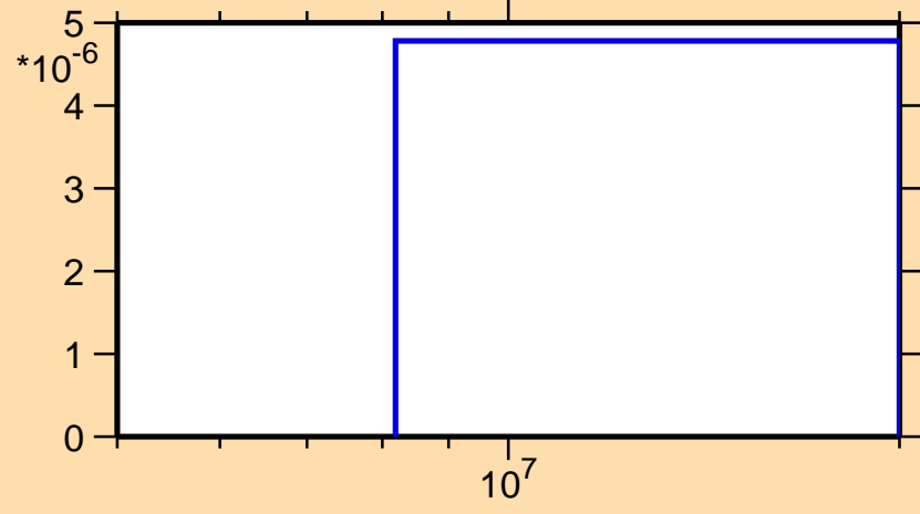
\sigma vs. E for ^{133}\text{Sb}(n,np)
