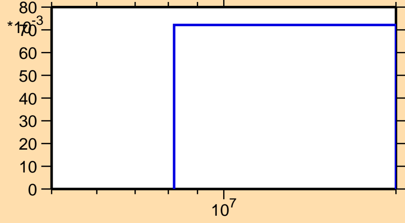
\sigma vs. E for ^{133}\text{Sb}(n,3n)
