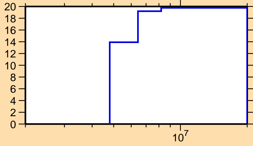
\Delta\sigma/\sigma vs. E for ^{133}\text{Sb}(n,\text{inel.})
