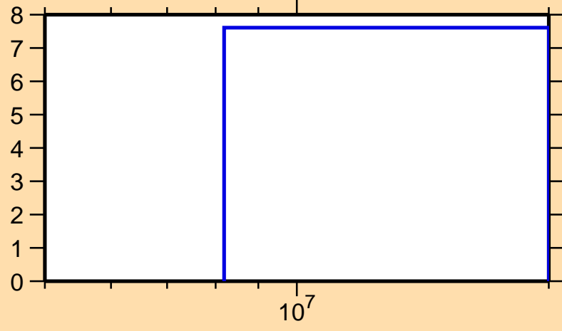
\Delta\sigma/\sigma vs. E for ^{133}\text{Sb}(n,\text{el.})
