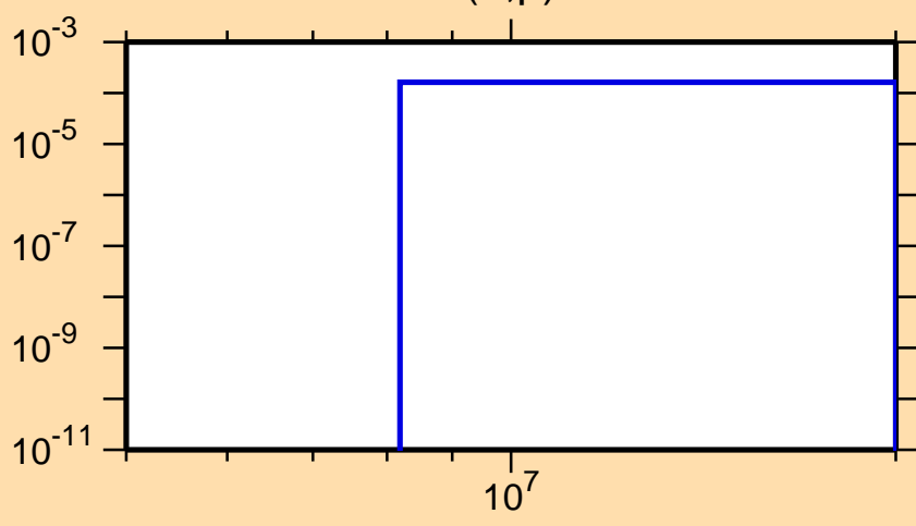
\sigma vs. E for ^{133}\text{Sb}(n,p)
