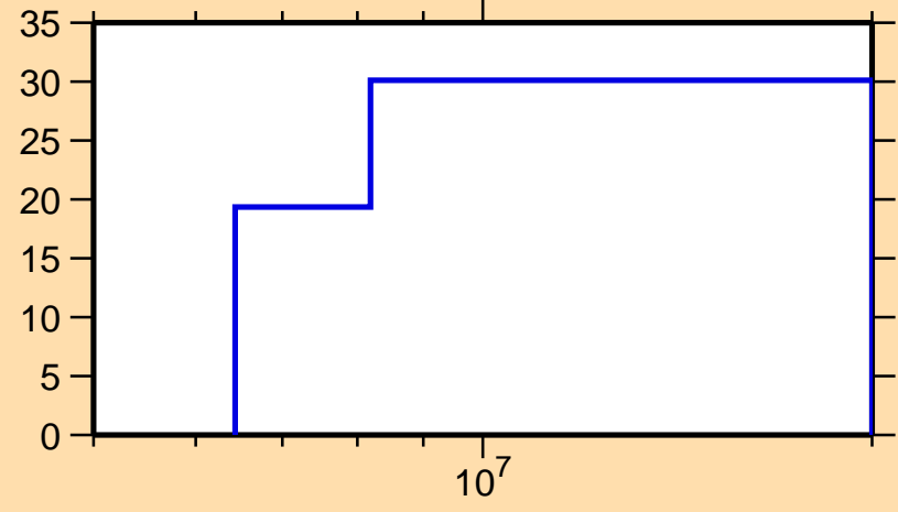
\Delta\sigma/\sigma vs. E for ^{133}\text{Sb}(n,ncont.)
