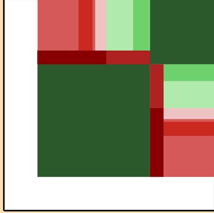
\sigma vs. E for ^{133}\text{Sb}(n,\text{inel.})
