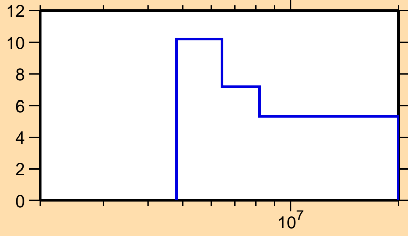
\Delta\sigma/\sigma vs. E for ^{133}\text{Sb}(n,\text{tot.})
