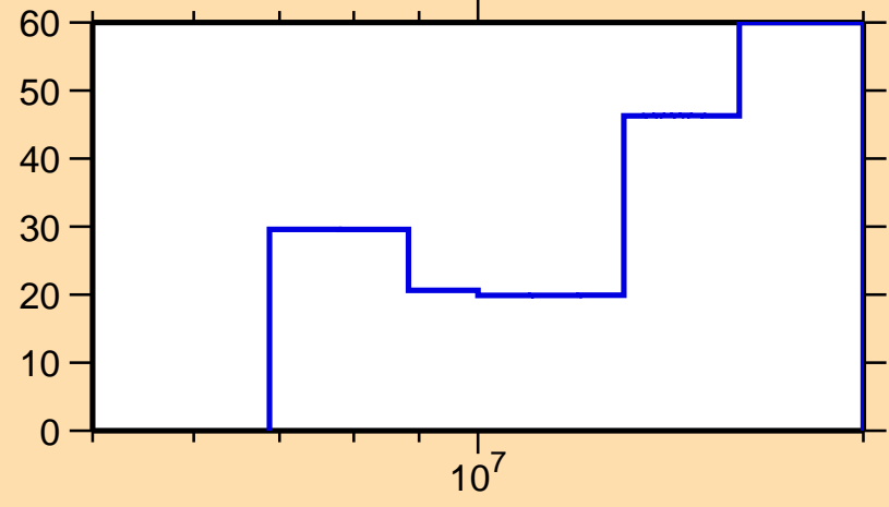
\Delta\sigma/\sigma vs. E for ^{134}\text{Sb}(n,2n)
