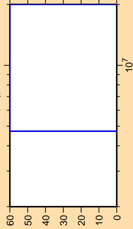
\Delta\sigma/\sigma vs. E for ^{134}\text{Sb}(n,\gamma)
