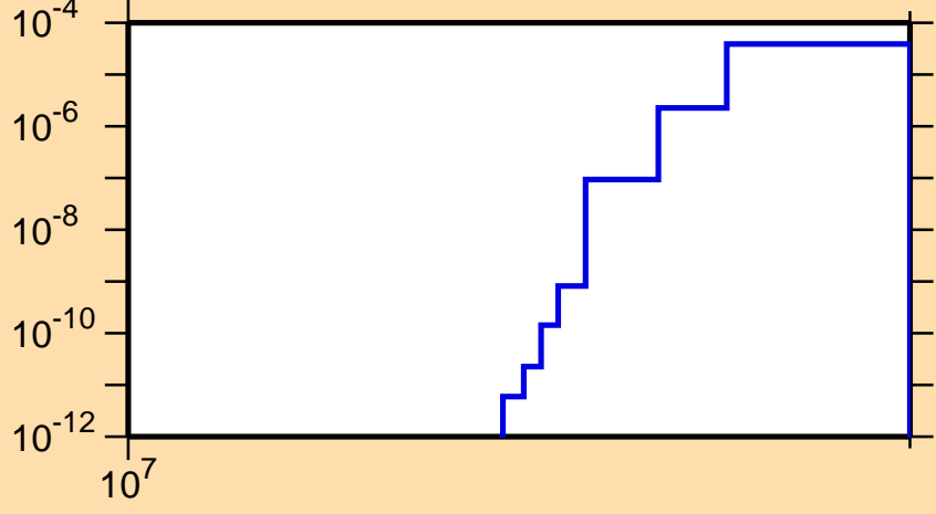
\sigma vs. E for ^{134}\text{Sb}(n,nt)
