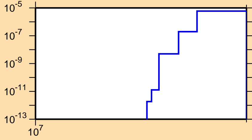
\sigma vs. E for ^{134}\text{Sb}(n,2np)
