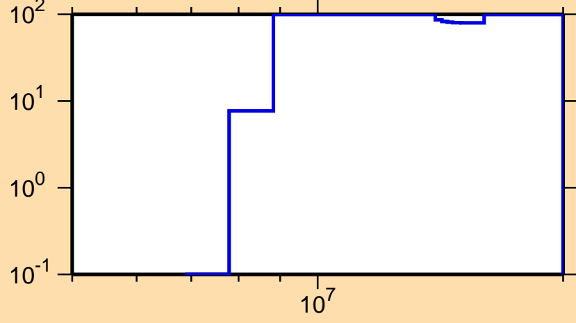
\Delta\sigma/\sigma vs. E for ^{134}\text{Sb}(n,p)
