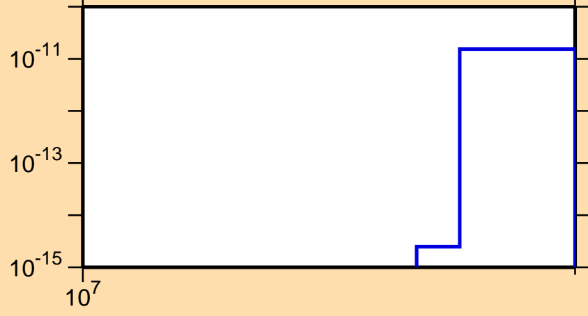
\sigma vs. E for ^{134}\text{Sb}(n,2n\alpha)
