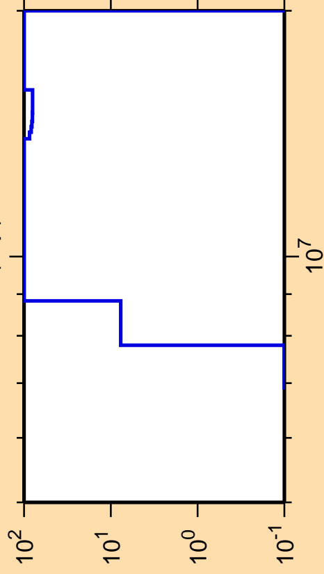
\Delta\sigma/\sigma vs. E for ^{134}\text{Sb}(n,p)
