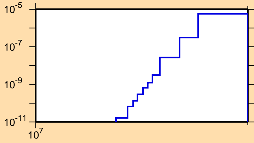
\sigma vs. E for ^{134}\text{Sb}(n,n\alpha)
