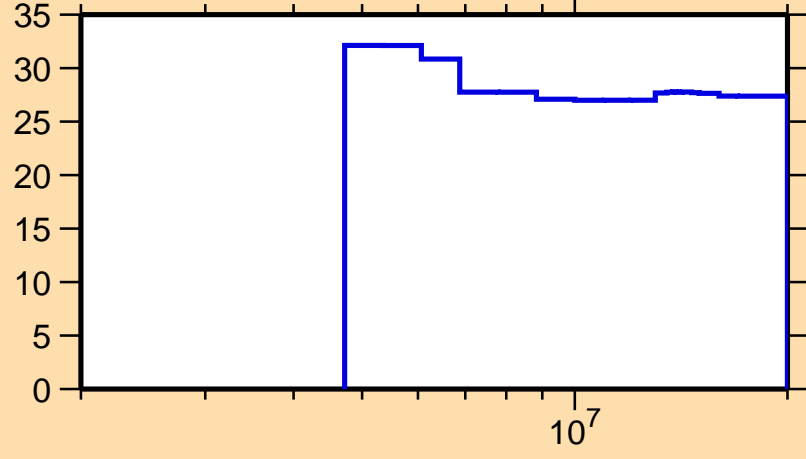
\Delta\sigma/\sigma vs. E for ^{134}\text{Sb}(n,n\text{onel.})
