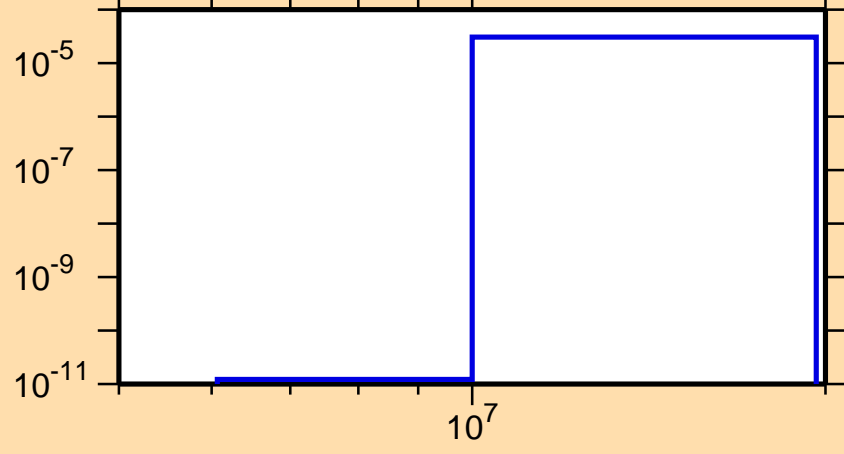
\sigma vs. E for ^{134}\text{Sb}(n,p)
