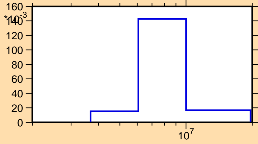
\sigma vs. E for ^{134}\text{Sb}(n,n\text{cont.})
