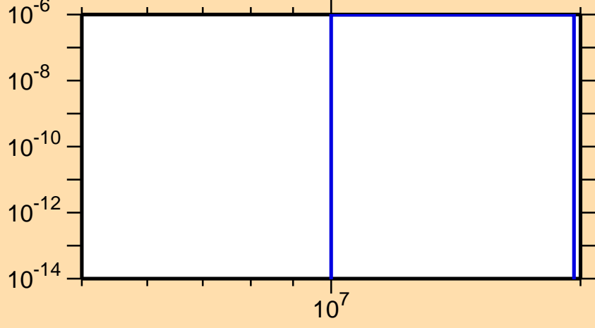
\sigma vs. E for ^{134}\text{Sb}(n,d)
