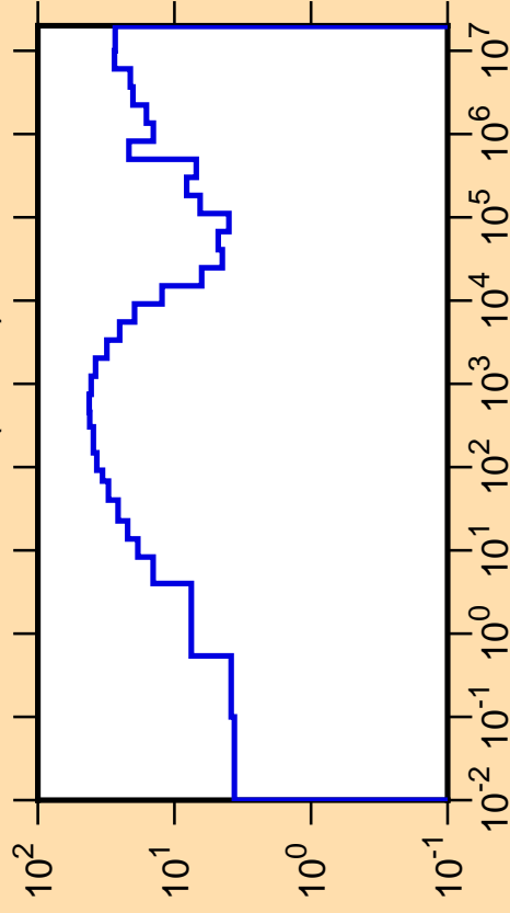
\Delta\sigma/\sigma vs. E for ^{134}\text{Sb}(n,\text{tot.})
