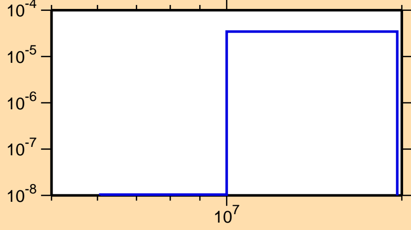
\sigma vs. E for ^{134}\text{Sb}(n,t)
