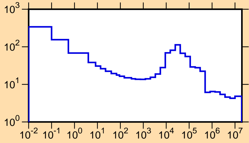
\sigma vs. E for ^{134}\text{Sb}(n,\text{tot.})
