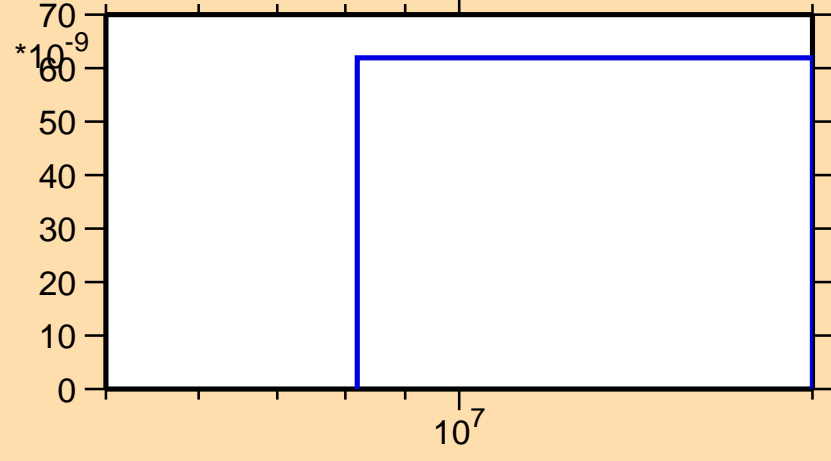
\sigma vs. E for ^{134}\text{Sb}(n,n\alpha)
