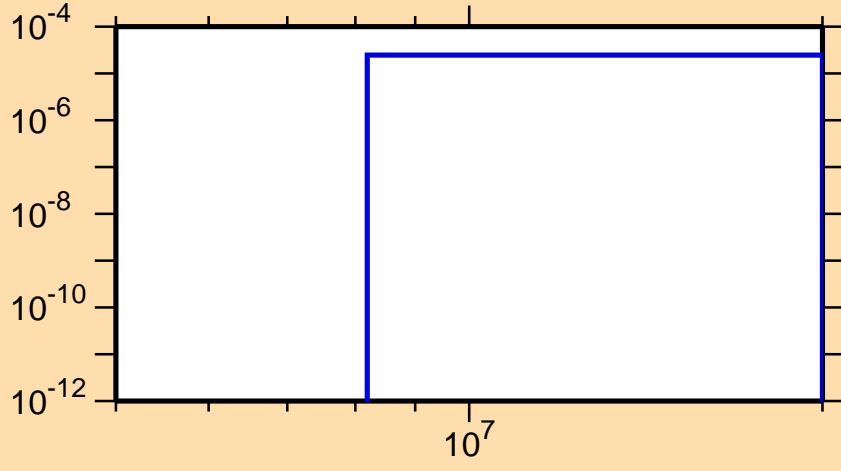
\sigma vs. E for ^{134}\text{Sb}(n,p)
