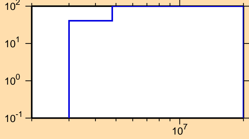
\Delta\sigma/\sigma vs. E for ^{134}\text{Sb}(n,n_1)
