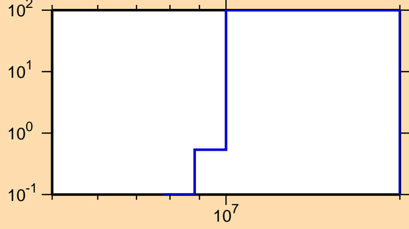
\Delta\sigma/\sigma vs. E for ^{135}\text{Sb}(n,p)
