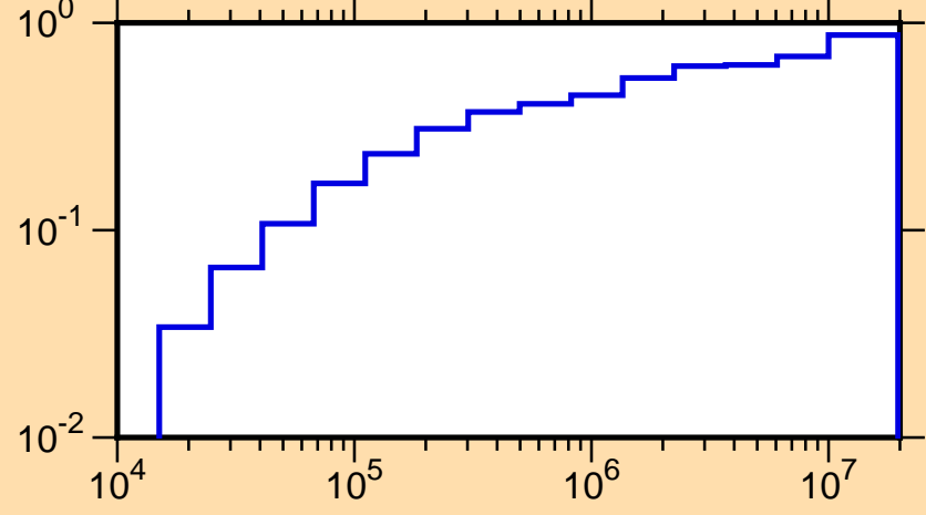
\mu vs. E for ^{135}\text{Sb}(\text{mt251})
