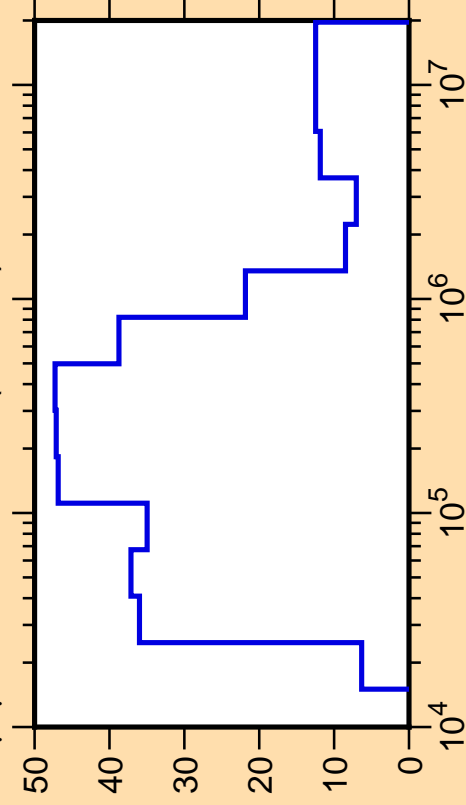
\Delta\mu/\mu vs. E for ^{135}\text{Sb}(\text{mt251})
