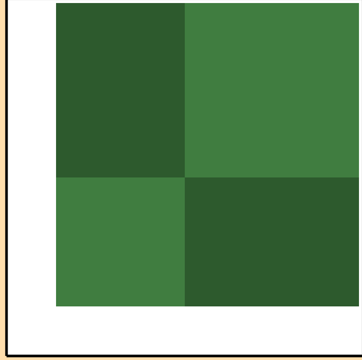
\Delta\sigma/\sigma vs. E for ^{135}\text{Sb}(n,p)
