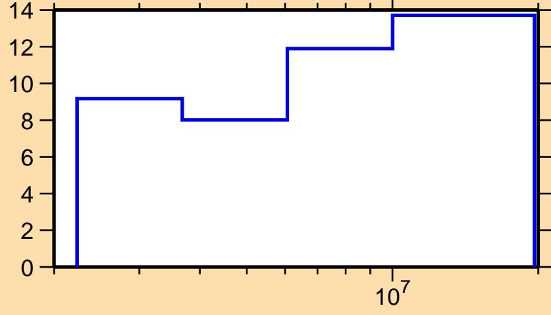
\Delta\sigma/\sigma vs. E for ^{135}\text{Sb}(n,n\text{nonel.})
