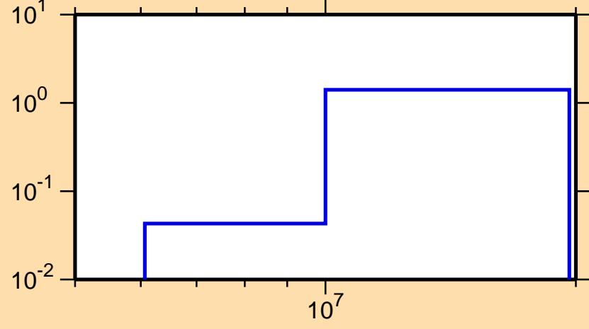
\sigma vs. E for ^{135}\text{Sb}(n,3n)
