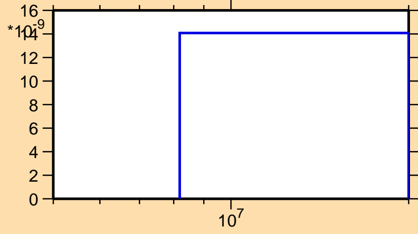
\sigma vs. E for ^{135}\text{Sb}(n,n\alpha)
