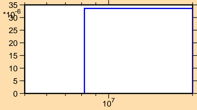
\sigma vs. E for ^{135}\text{Sb}(n,d)
