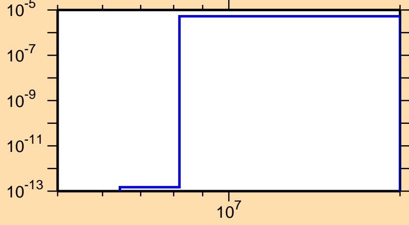
\sigma vs. E for ^{135}\text{Sb}(n,\alpha)
