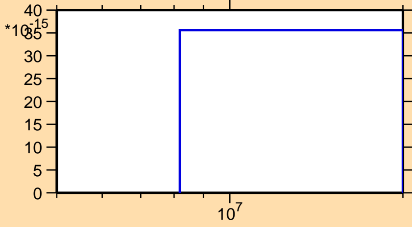
\sigma vs. E for ^{135}\text{Sb} (mt 42)
