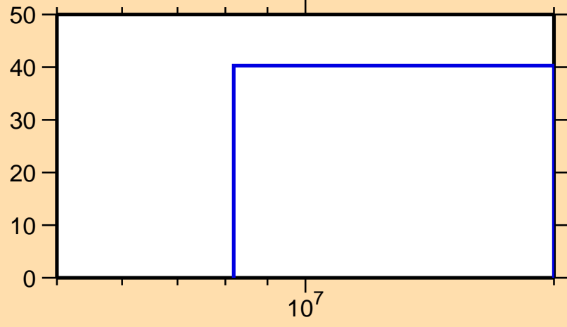
\Delta\sigma/\sigma vs. E for ^{135}\text{Sb}(n,\text{inel.})
