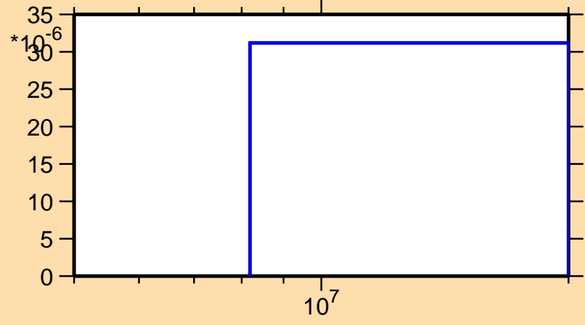
\sigma vs. E for ^{135}\text{Sb}(n,nt)
