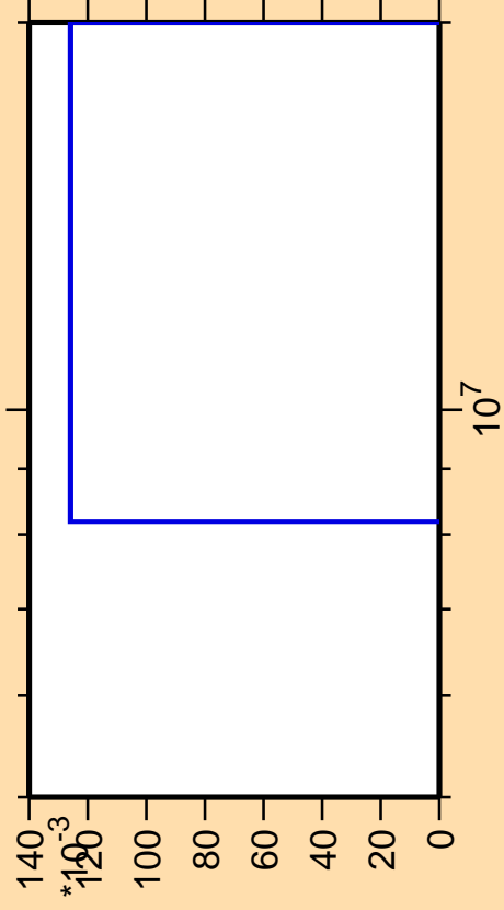
\Delta\sigma/\sigma vs. E for ^{135}\text{Sb} (mt 42)
