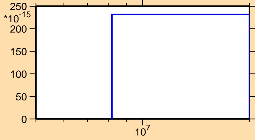
\sigma vs. E for ^{135}\text{Sb}(n,2n\alpha)
