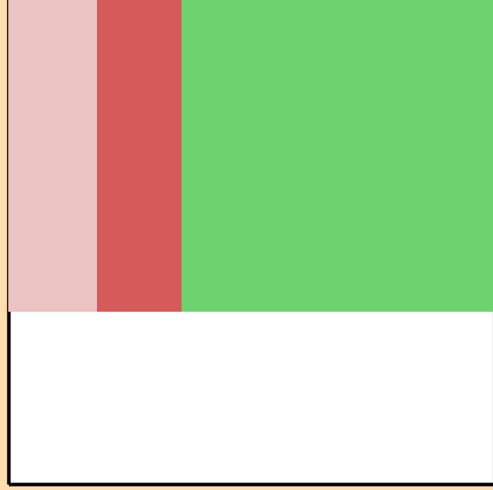
\Delta\sigma/\sigma vs. E for ^{135}\text{Sb}(n,\gamma)
