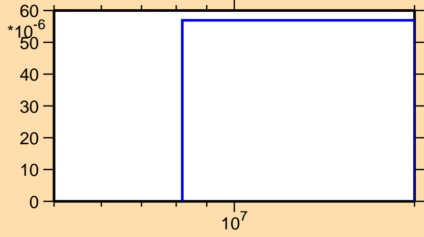
\sigma vs. E for ^{135}\text{Sb}(n,p)
