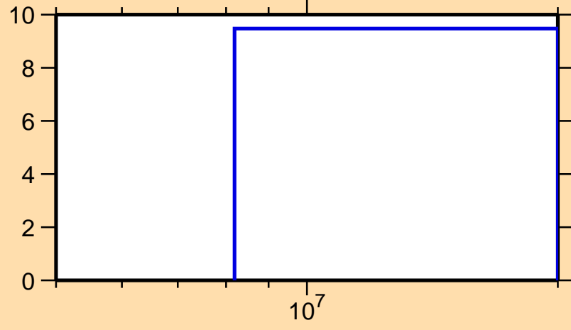
\Delta\sigma/\sigma vs. E for ^{135}\text{Sb}(n,el.)
