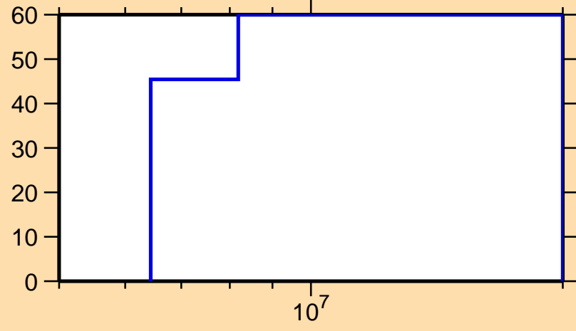
\Delta\sigma/\sigma vs. E for ^{135}\text{Sb}(n,n\text{cont.})
