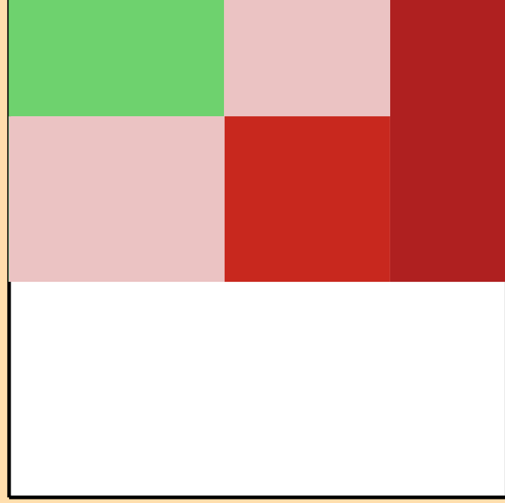
\Delta\sigma/\sigma vs. E for ^{43}\text{Sc}(n,\text{el.})
