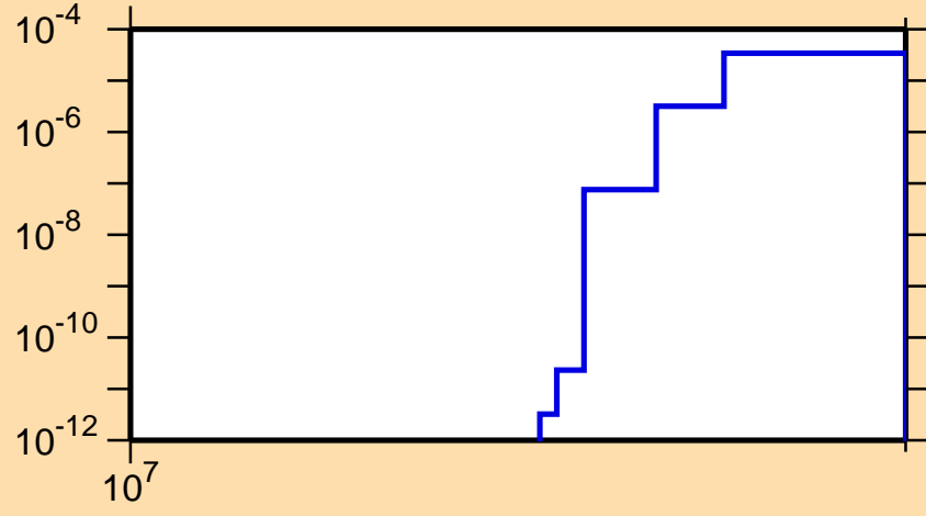
\sigma vs. E for ^{43}\text{Sc}(n,\text{pd})
