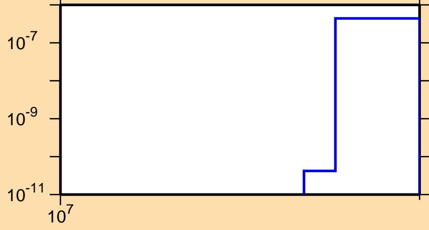
\sigma vs. E for ^{43}\text{Sc}(n,nt)
