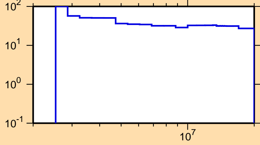
\Delta\sigma/\sigma vs. E for ^{43}\text{Sc}(n,n\text{cont.})
