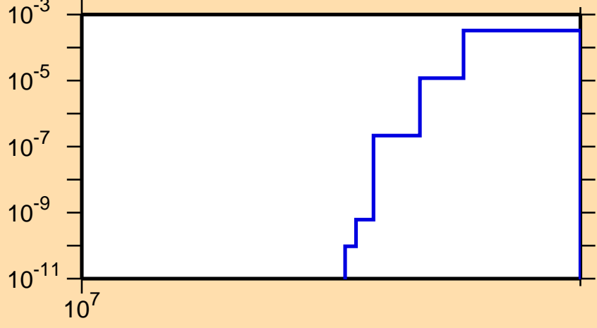
\sigma vs. E for ^{43}\text{Sc}(\text{mt } 45)
