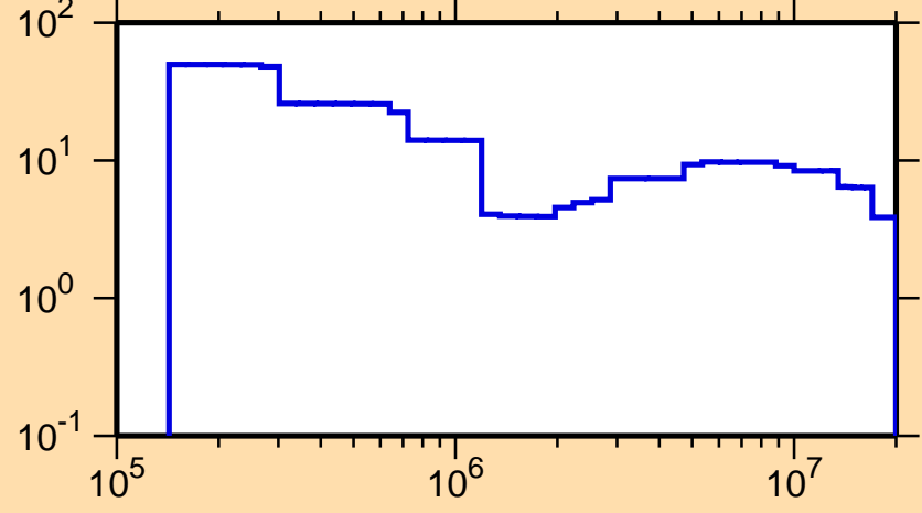
\Delta\sigma/\sigma vs. E for ^{43}\text{Sc}(n,\text{tot.})
