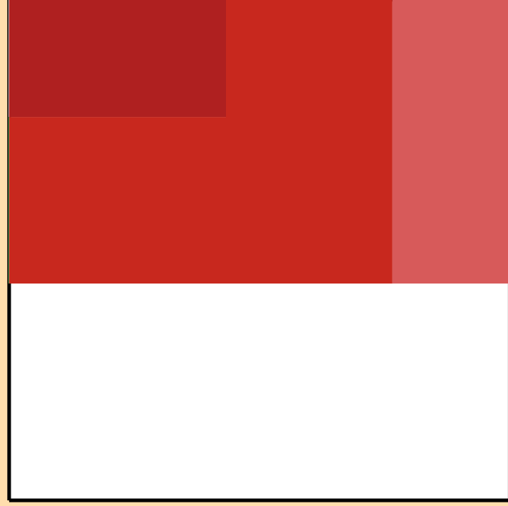
\Delta\sigma/\sigma vs. E for ^{43}\text{Sc}(n,\text{inel.})
