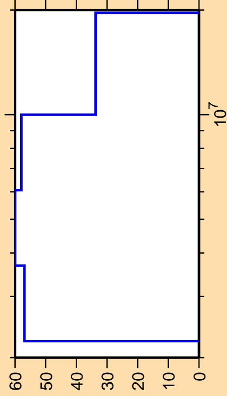
\Delta\sigma/\sigma vs. E for ^{43}\text{Sc}(n,d)
