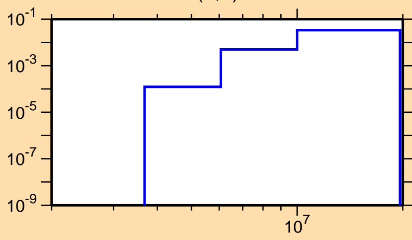
\sigma vs. E for ^{43}\text{Sc}(n,d)
