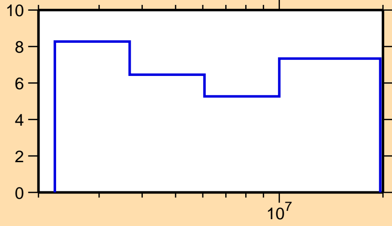
\Delta\sigma/\sigma vs. E for ^{43}\text{Sc}(n,n\text{onel.})
