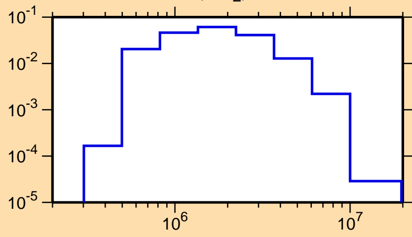
\sigma vs. E for ^{43}\text{Sc}(n,n_2)
