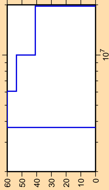
\Delta\sigma/\sigma vs. E for ^{43}\text{Sc}(n,np)
