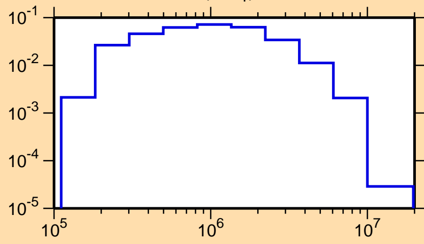
\sigma vs. E for ^{43}\text{Sc}(n,n_1)
