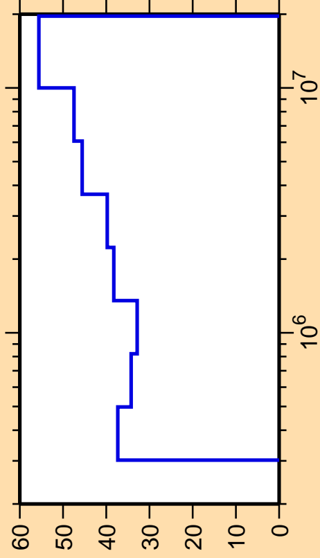
\Delta\sigma/\sigma vs. E for ^{43}\text{Sc}(n,n_2)
