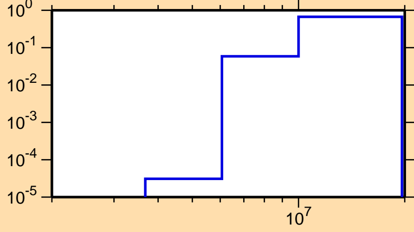
\sigma vs. E for ^{43}\text{Sc}(n,np)
