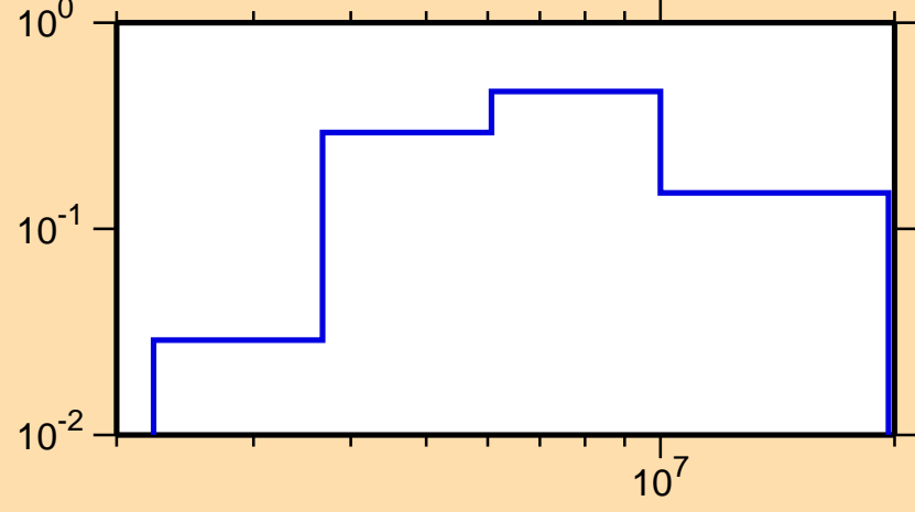
\sigma vs. E for ^{43}\text{Sc}(n,n\text{cont.})
