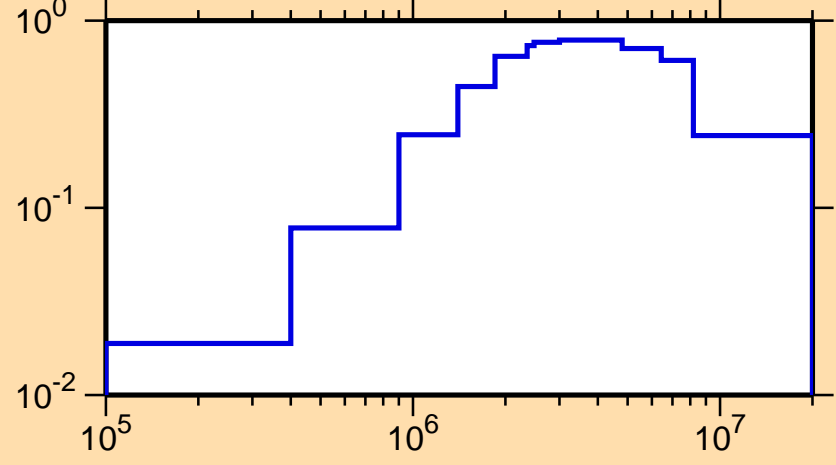
\sigma vs. E for ^{43}\text{Sc}(n,\text{inel.})
