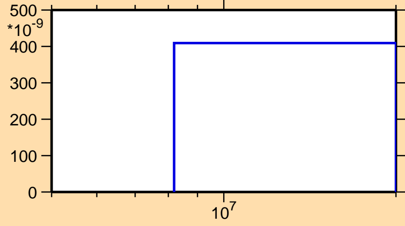
\sigma vs. E for ^{43}\text{Sc}(n,pd)
