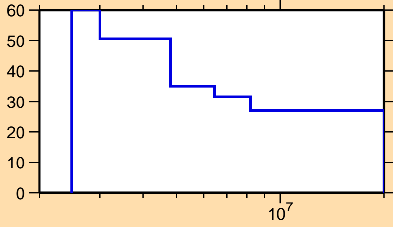
\Delta\sigma/\sigma vs. E for ^{43}\text{Sc}(n,n\text{cont.})
