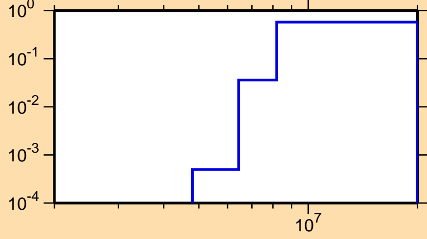
\sigma vs. E for ^{43}\text{Sc}(n,np)
