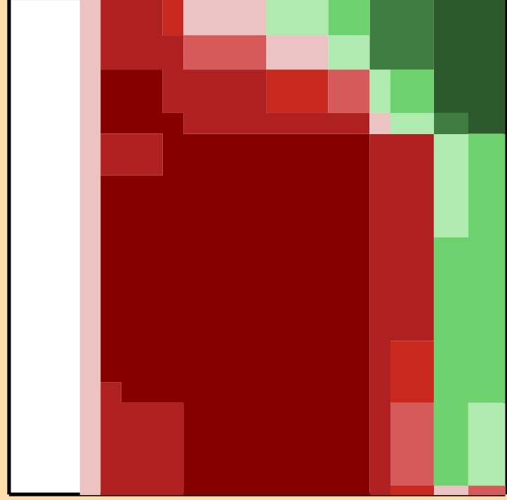
\Delta\sigma/\sigma vs. E for ^{44}\text{Sc}(n,ncont.)
