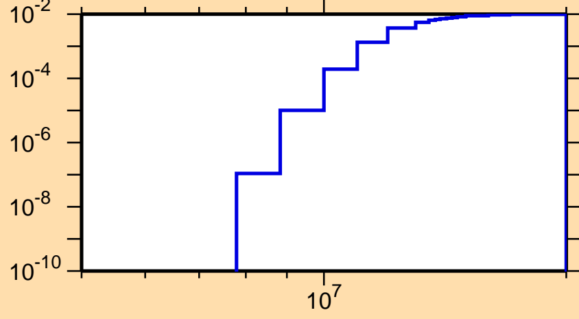
\sigma vs. E for ^{44}\text{Sc}(n,p\alpha)
