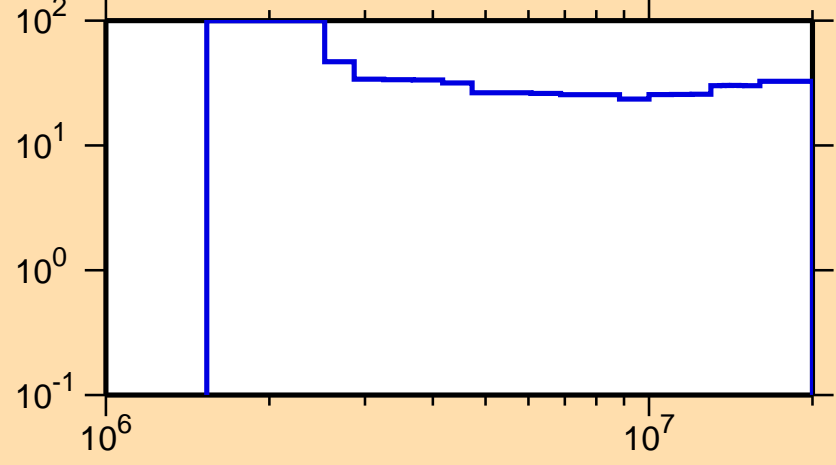
\Delta\sigma/\sigma vs. E for ^{44}\text{Sc}(n,n\text{cont.})
