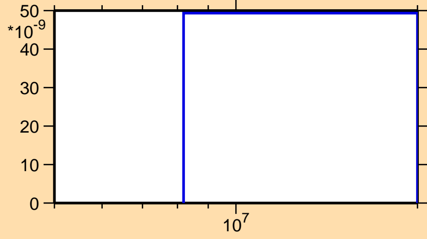
\sigma vs. E for ^{44}\text{Sc}(n,2n\alpha)
