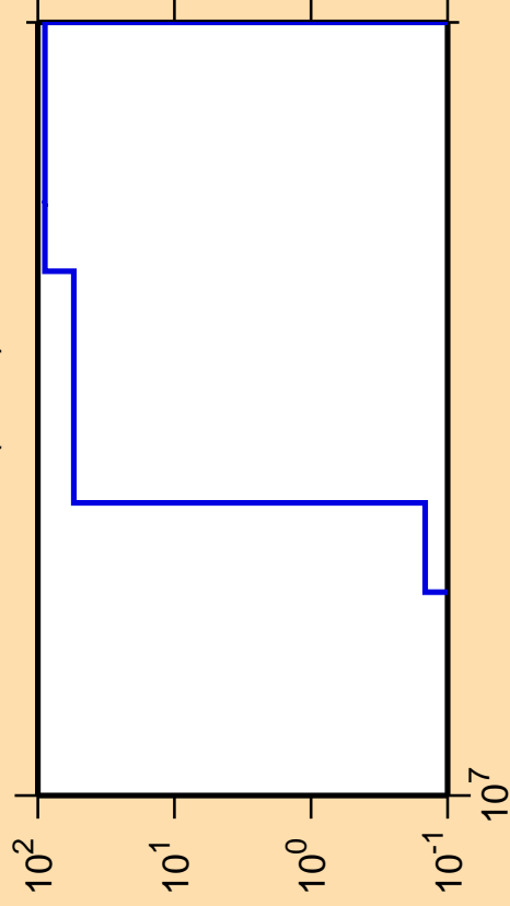
\Delta\sigma/\sigma vs. E for ^{44}\text{Sc}(n,nd)
