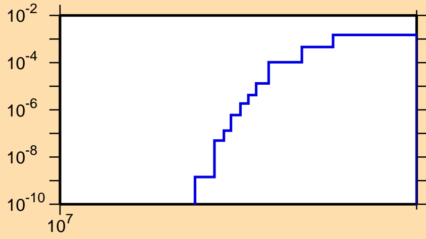
\sigma vs. E for ^{44}\text{Sc}(n,nd)
