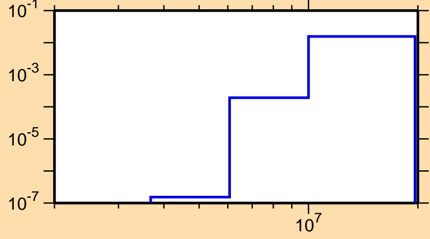
\sigma vs. E for ^{44}\text{Sc}(n,d)
