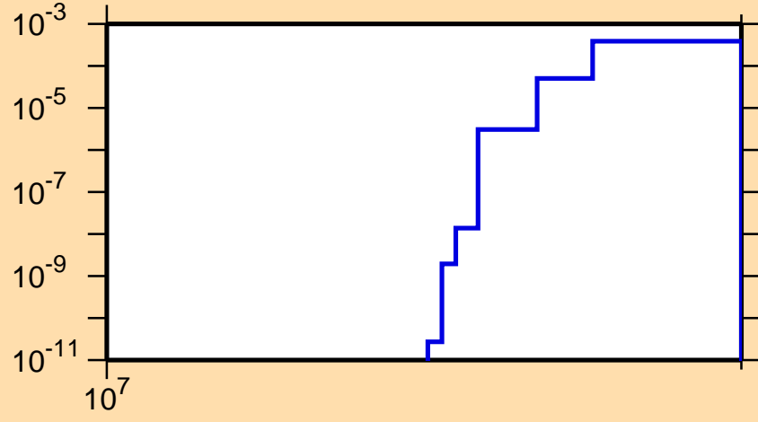
\sigma vs. E for ^{46}\text{Sc}(n,nd)
