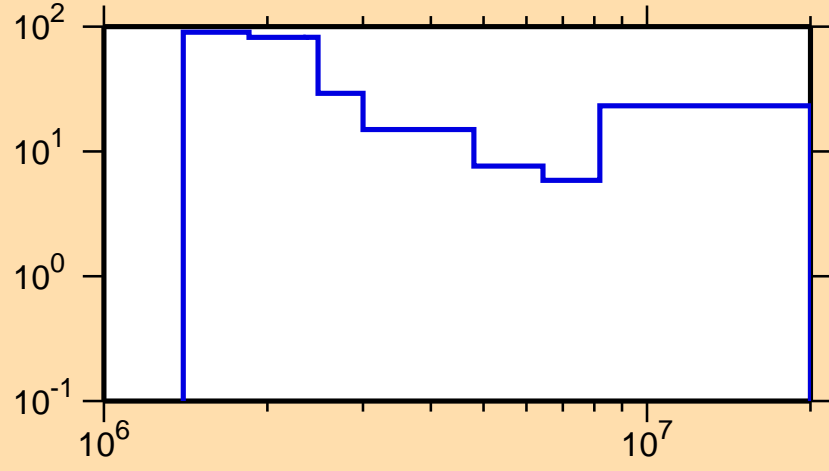
\Delta\sigma/\sigma vs. E for ^{46}\text{Sc}(n,ncont.)
