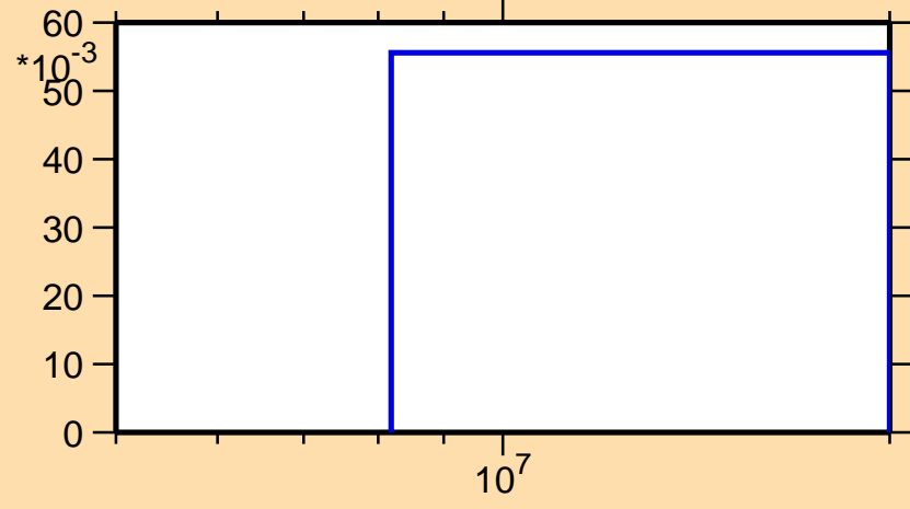
\sigma vs. E for ^{46}\text{Sc}(n,np)
