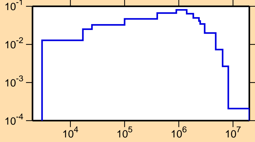
\sigma vs. E for ^{46}\text{Sc}(n,n_1)
