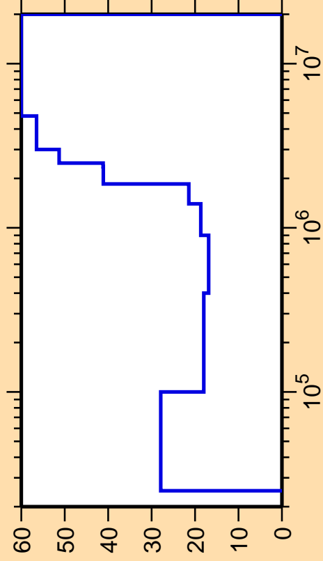
\Delta\sigma/\sigma vs. E for ^{46}\text{Sc}(n,n_3)
