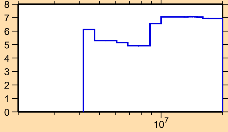
\Delta\sigma/\sigma vs. E for ^{47}\text{Sc}(n,\text{nonel.})
