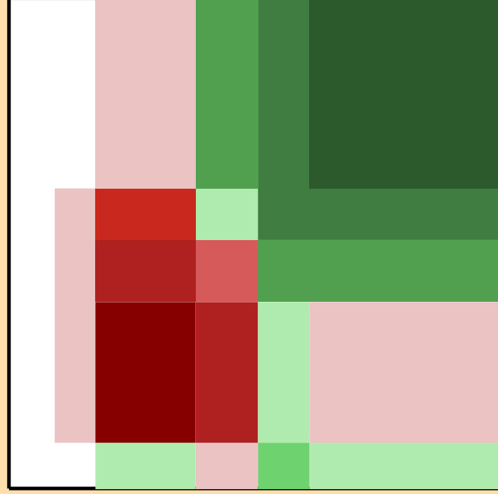
\Delta\sigma/\sigma vs. E for ^{47}\text{Sc}(n,ncont.)
