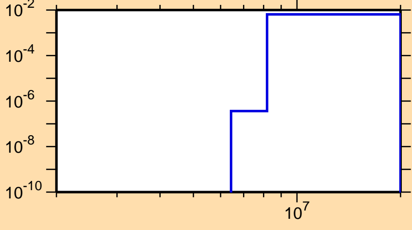
\sigma vs. E for ^{47}\text{Sc}(n,d)
