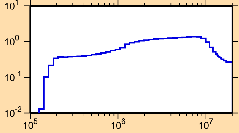
\sigma vs. E for ^{48}\text{Sc}(n,\text{inel.})
