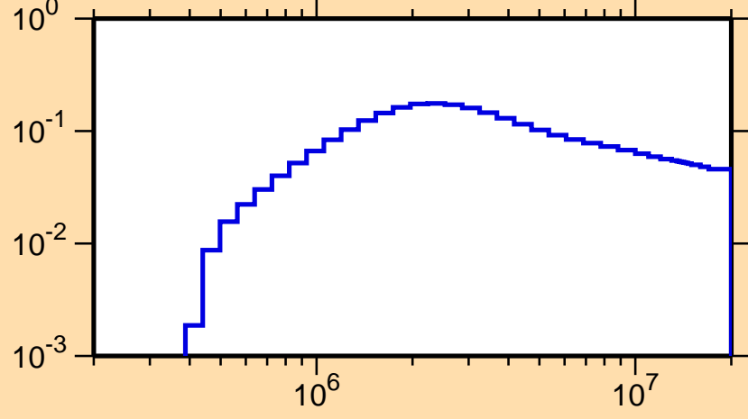
\sigma vs. E for ^{48}\text{Sc}(n,n_3)
