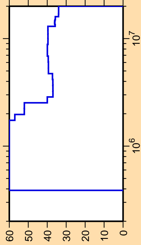
\Delta\sigma/\sigma vs. E for ^{48}\text{Sc}(n,n_3)
