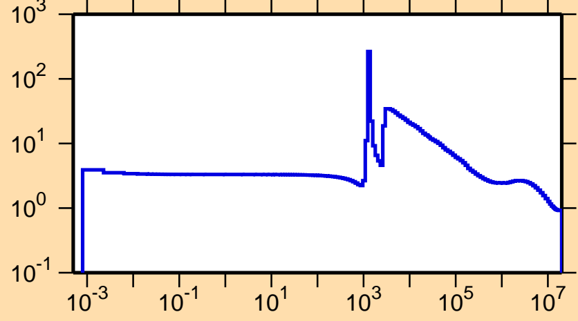
\sigma vs. E for ^{48}\text{Sc}(n,\text{el.})
