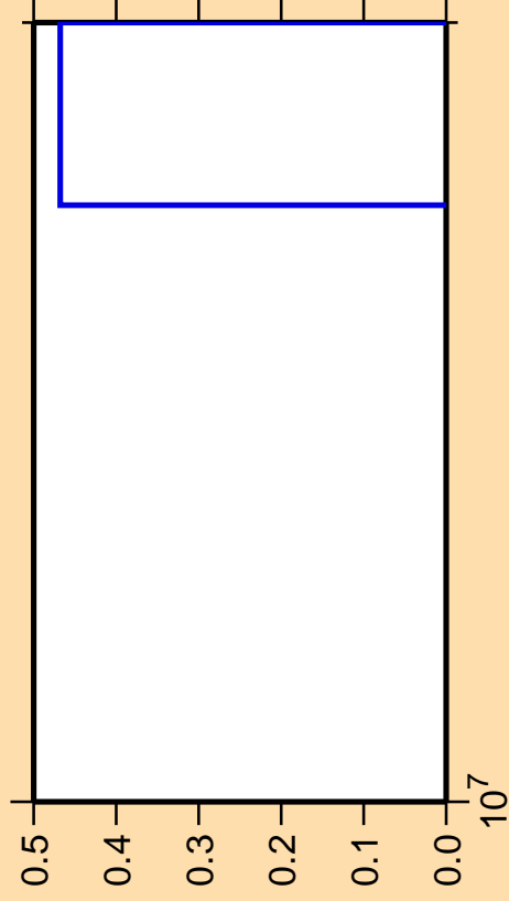
\Delta\sigma/\sigma vs. E for ^{48}\text{Sc}(n,nt)
