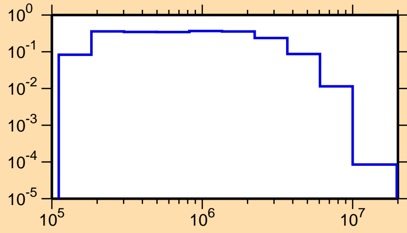
\sigma vs. E for ^{48}\text{Sc}(n,n_1)
