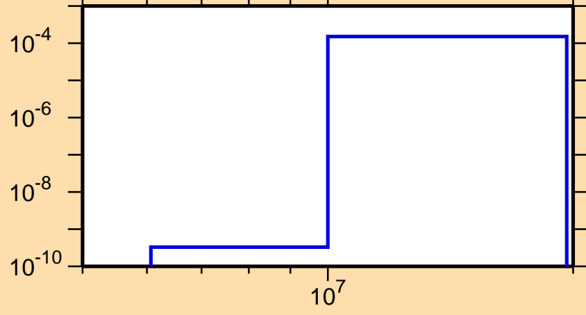
\sigma vs. E for ^{48}\text{Sc}(n,t)
