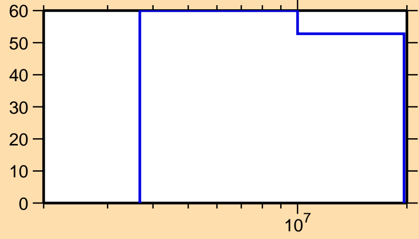
\Delta\sigma/\sigma vs. E for ^{50}\text{Sc}(n,\gamma)
