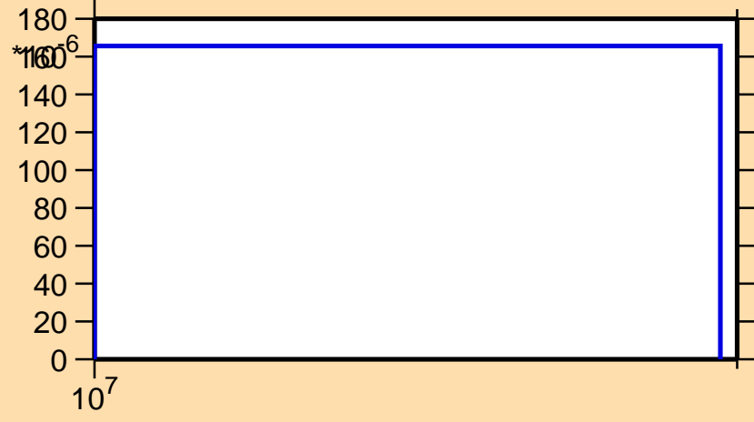
\sigma vs. E for ^{50}\text{Sc}(n,3n)
