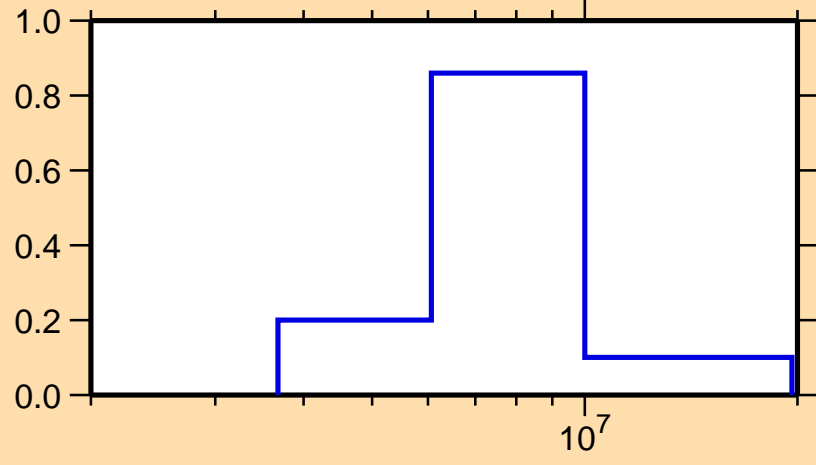
\sigma vs. E for ^{50}\text{Sc}(n,n\text{cont.})
