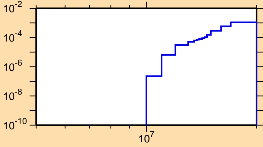
\sigma vs. E for ^{51}\text{Sc}(n,t)
