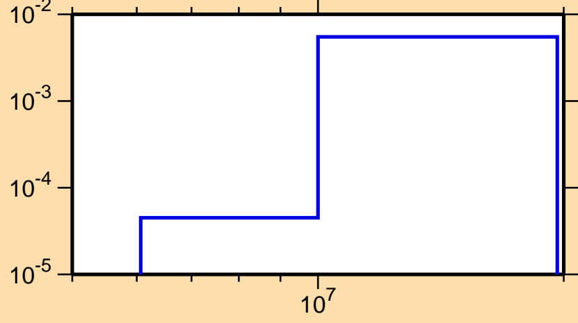
\sigma vs. E for ^{51}\text{Sc}(n,p)
