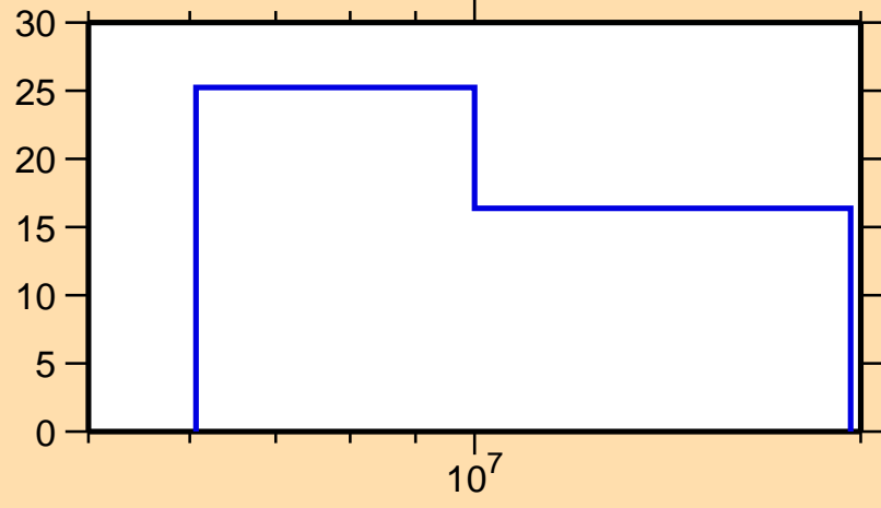
\Delta\sigma/\sigma vs. E for ^{51}\text{Sc}(n,el.)
