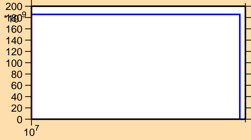
\sigma vs. E for ^{51}\text{Sc}(n,\text{nd})
