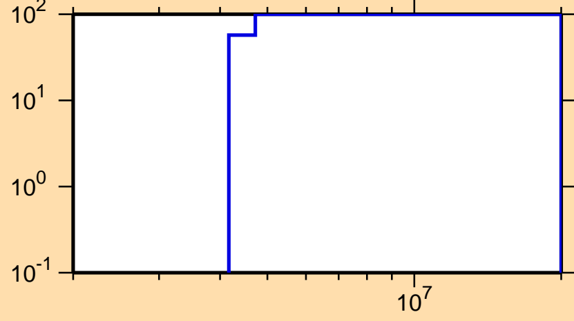
\Delta\sigma/\sigma vs. E for ^{52}\text{Sc}(n,n_1)
