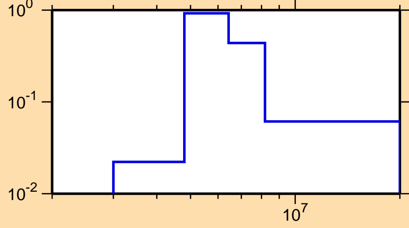
\sigma vs. E for ^{52}\text{Sc}(n,n\text{cont.})
