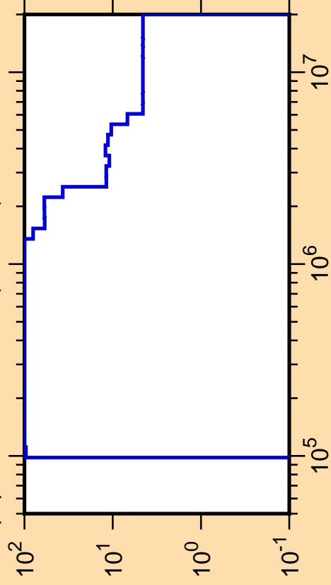
\Delta\mu/\mu vs. E for ^{53}\text{Sc}(\text{mt251})
