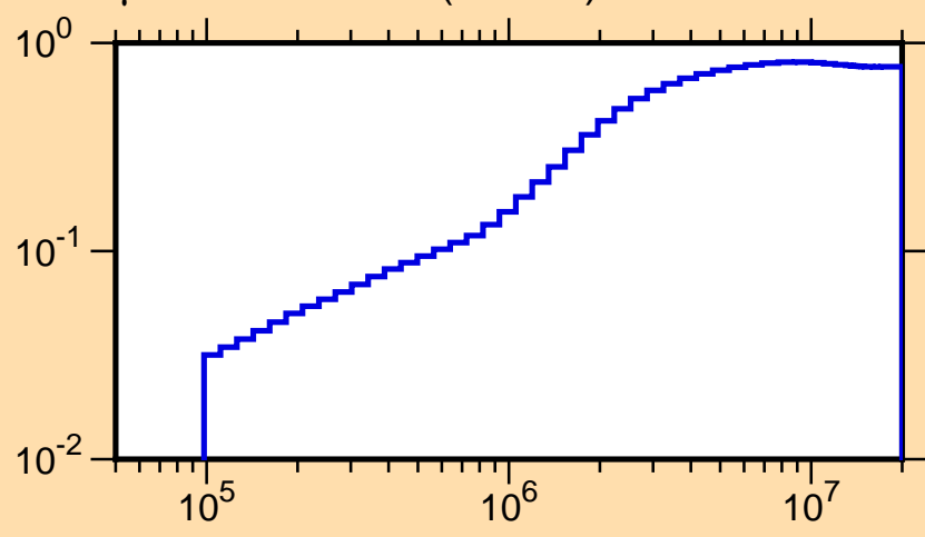
\mu vs. E for ^{53}\text{Sc}(\text{mt251})
