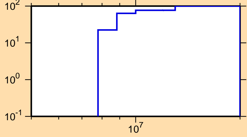
\Delta\sigma/\sigma vs. E for ^{53}\text{Sc}(n,ncont.)
