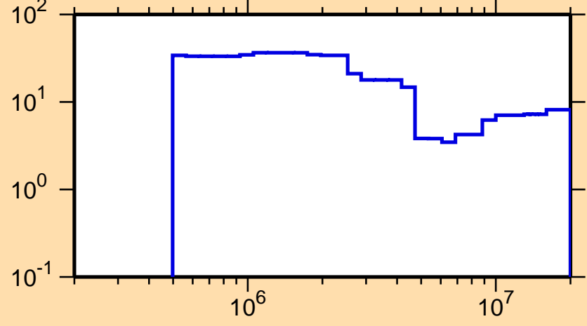
\Delta\sigma/\sigma vs. E for ^{53}\text{Sc}(n,\text{nonel.})
