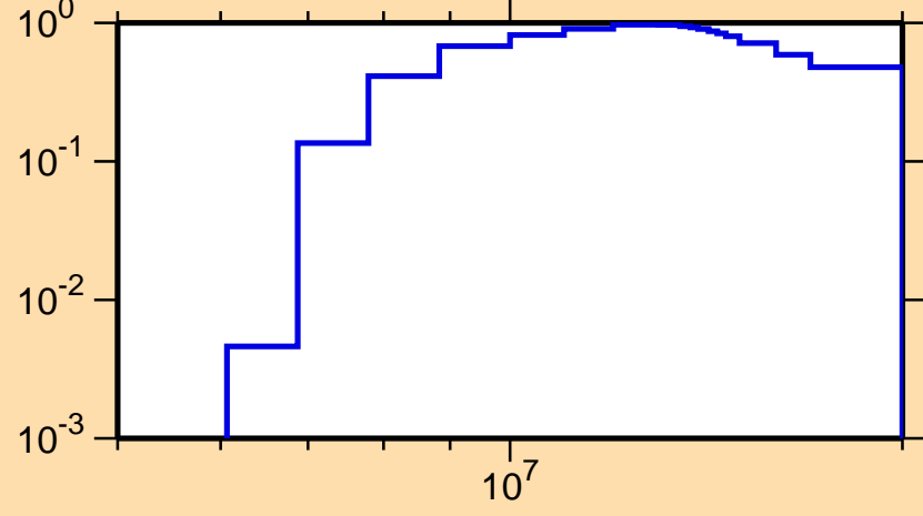
\sigma vs. E for ^{53}\text{Sc}(n,2n)
