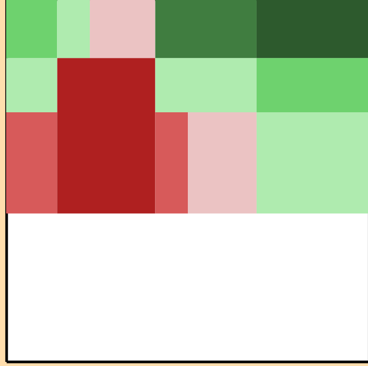
\Delta\sigma/\sigma vs. E for ^{53}\text{Sc}(n,ncont.)
