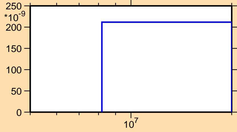
\sigma vs. E for ^{53}\text{Sc}(n,\alpha)
