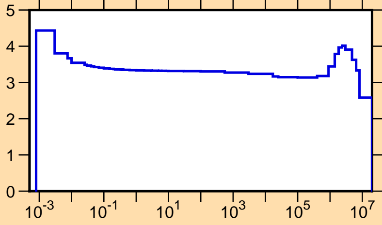
\sigma vs. E for ^{53}\text{Sc}(n,\text{tot.})
