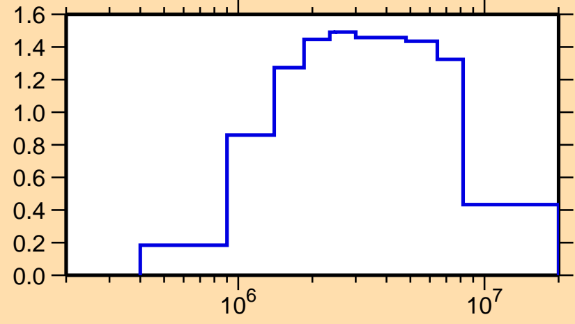
\sigma vs. E for ^{53}\text{Sc}(n,\text{inel.})
