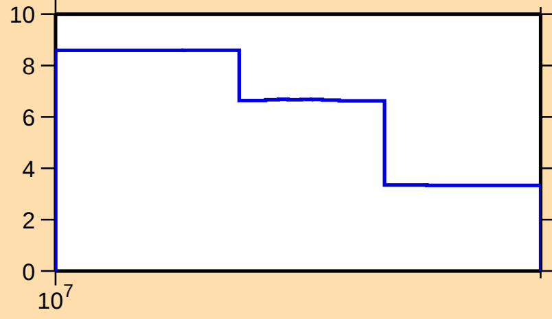
\Delta\sigma/\sigma vs. E for ^{69}\text{Se}(n,\text{tot.})
