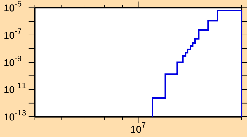
\sigma vs. E for ^{69}\text{Se}(\text{mt117})
