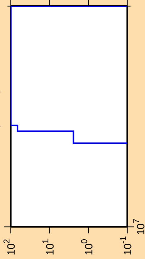
\Delta\sigma/\sigma vs. E for ^{69}\text{Se}(\text{mt } 34)
