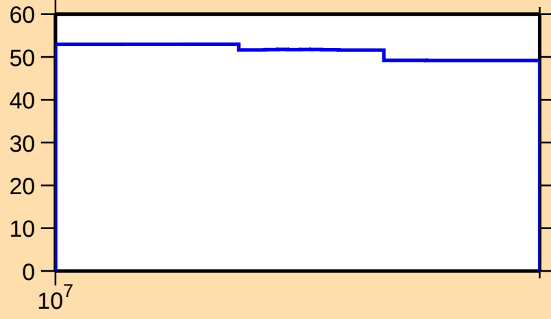
\Delta\sigma/\sigma vs. E for ^{69}\text{Se}(n,\text{inel.})
