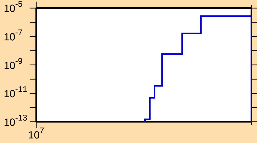
\sigma vs. E for ^{69}\text{Se}(n,\text{nd})
