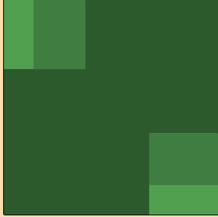
\sigma vs. E for ^{69}\text{Se}(n,2n)
