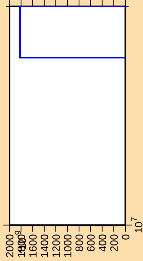
\Delta\sigma/\sigma vs. E for ^{69}\text{Se}(n,\text{nt})
