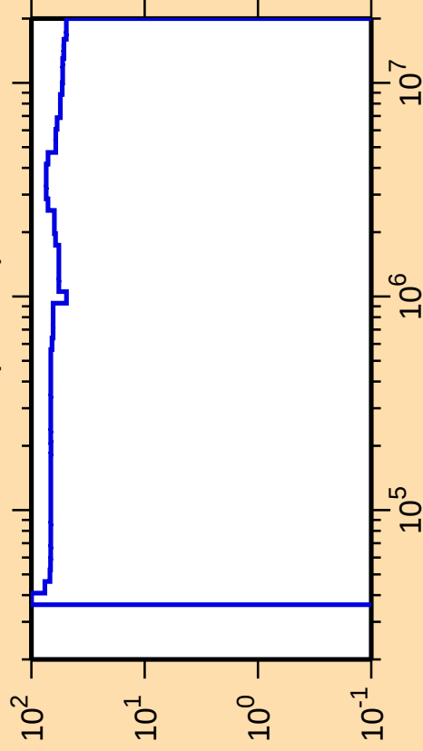
\Delta\sigma/\sigma vs. E for ^{69}\text{Se}(n,\text{inel.})
