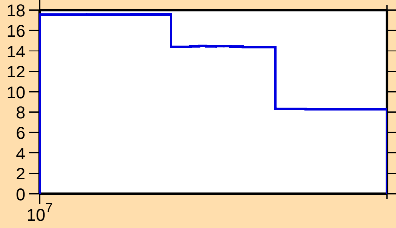
\Delta\sigma/\sigma vs. E for ^{69}\text{Se}(n,\text{el.})
