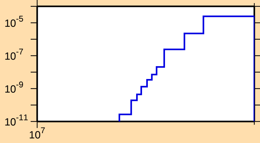
\sigma vs. E for ^{69}\text{Se}(\text{mt } 45)
