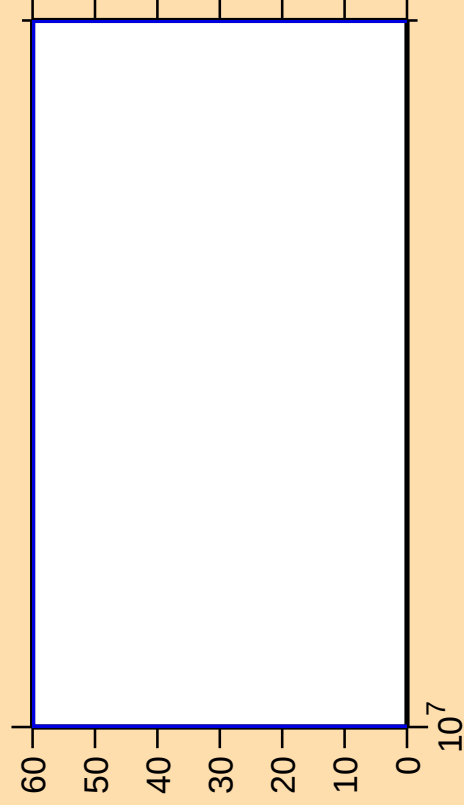
\Delta\sigma/\sigma vs. E for ^{69}\text{Se}(n,p)
