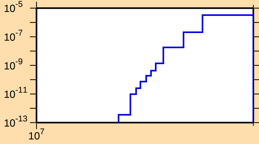
\sigma vs. E for ^{69}\text{Se}(\text{mt } 34)
