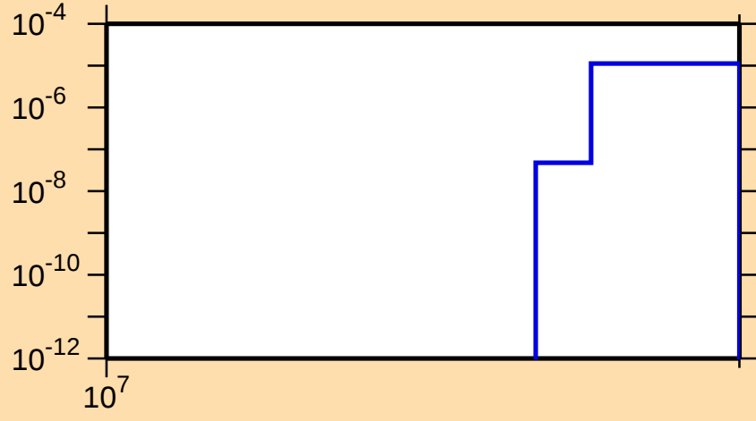
\sigma vs. E for ^{69}\text{Se}(n,2np)
