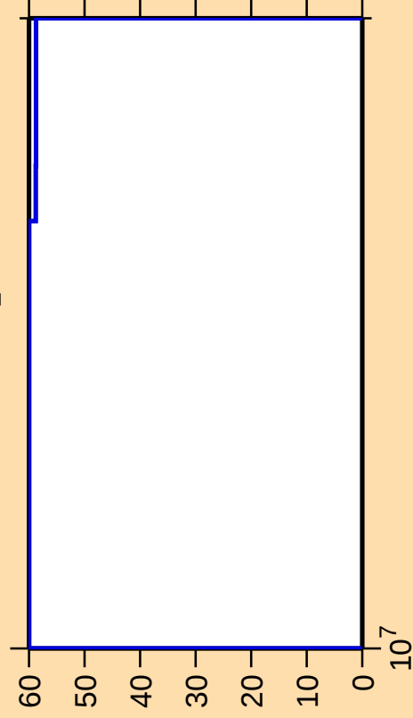
\Delta\sigma/\sigma vs. E for ^{69}\text{Se}(n,n_1)
