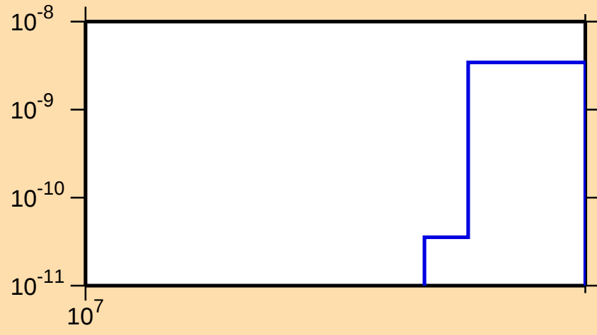
\sigma vs. E for ^{69}\text{Se}(n,2n\alpha)
