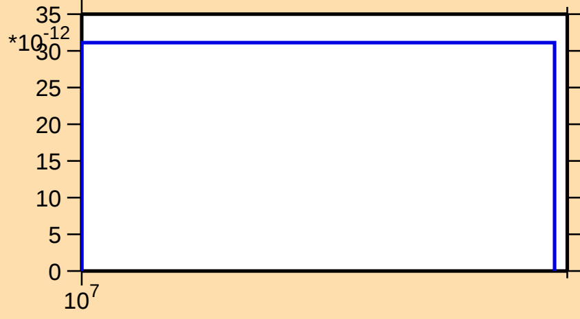
\sigma vs. E for ^{69}\text{Se}(n,2n\alpha)
