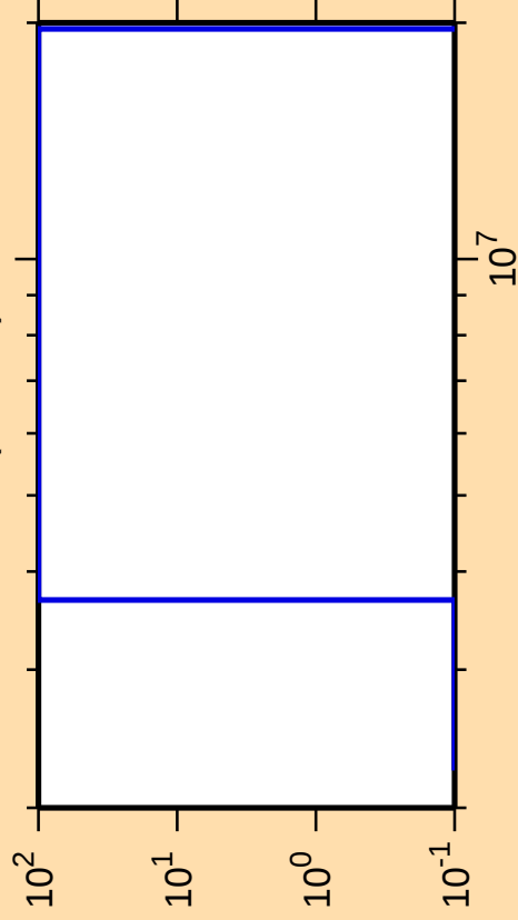
\Delta\sigma/\sigma vs. E for ^{69}\text{Se}(n,\text{He3})
