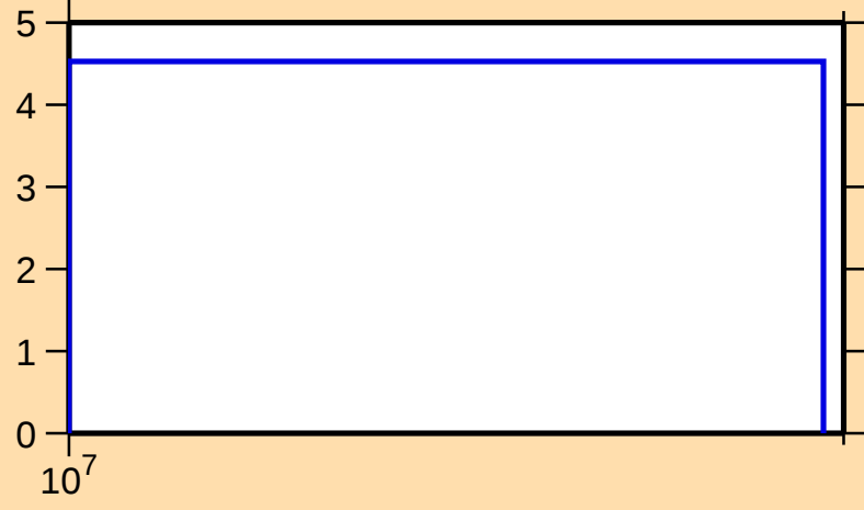
\Delta\sigma/\sigma vs. E for ^{69}\text{Se}(n,\text{nonel.})
