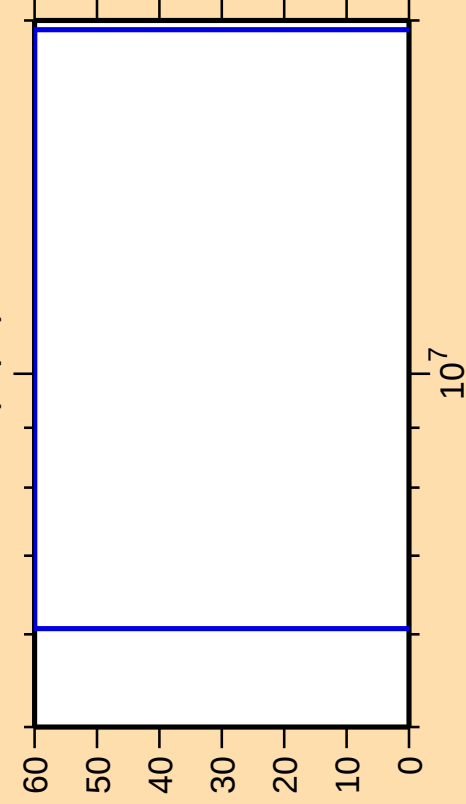
\Delta\sigma/\sigma vs. E for ^{69}\text{Se}(n,\text{pd})
