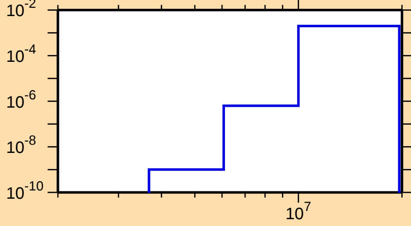
\sigma vs. E for ^{69}\text{Se}(n,\text{He3})
