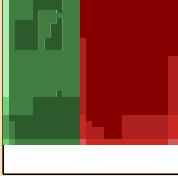
\Delta\sigma/\sigma vs. E for ^{72}\text{Se}(n,\text{nonel.})
