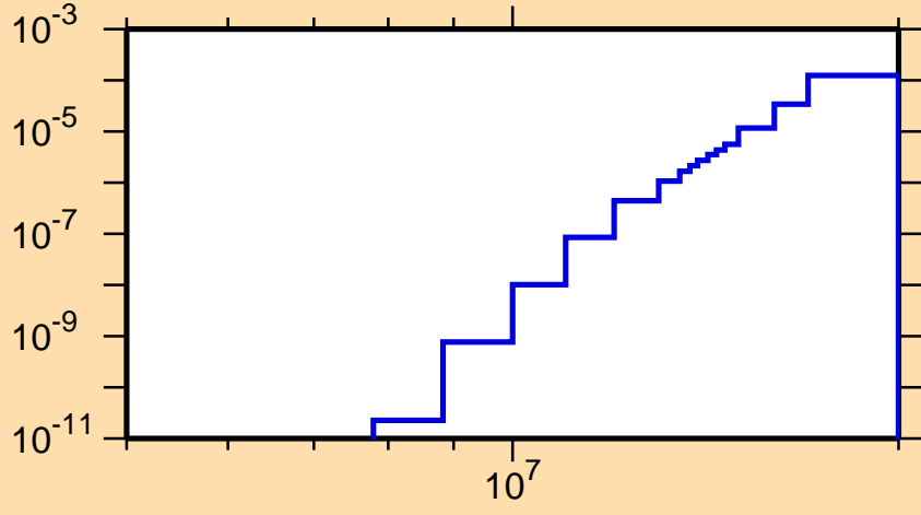
\sigma vs. E for ^{72}\text{Se}(n,\text{He3})
