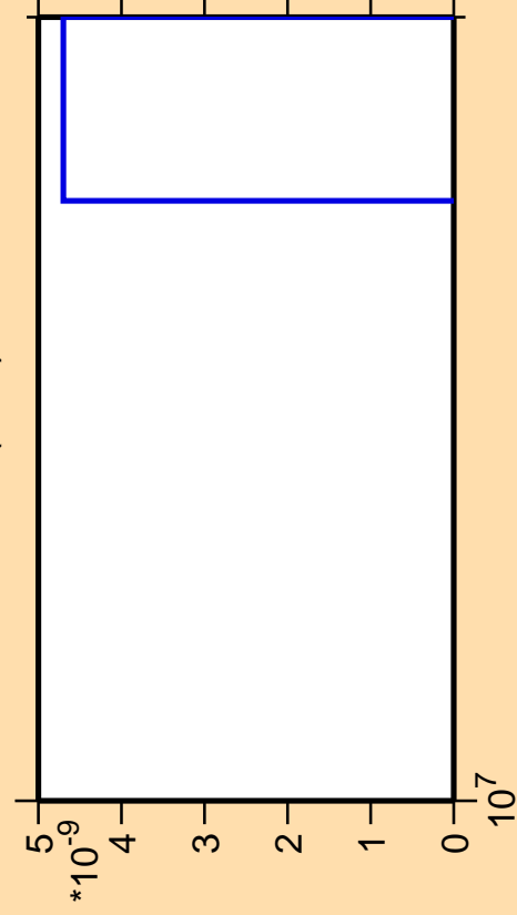
\Delta\sigma/\sigma vs. E for ^{72}\text{Se}(n,nt)
