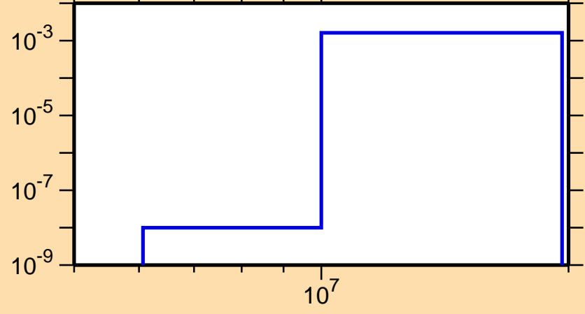
\sigma vs. E for ^{72}\text{Se}(n,p\alpha)
