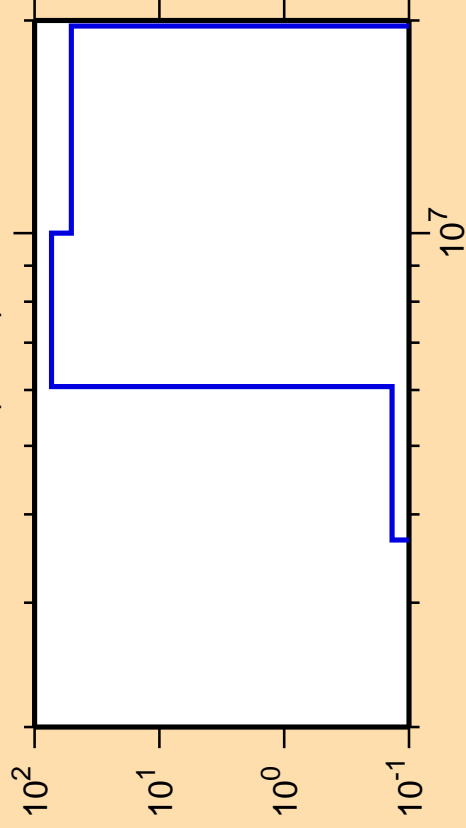
\Delta\sigma/\sigma vs. E for ^{72}\text{Se}(n,n\alpha)
