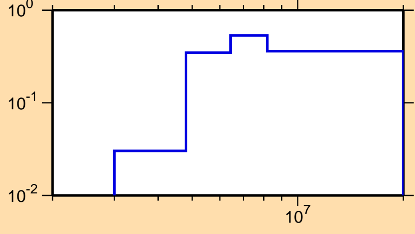
\sigma vs. E for ^{72}\text{Se}(n,n\text{cont.})
