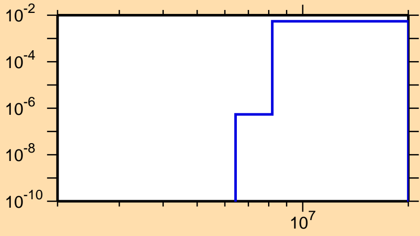
\sigma vs. E for ^{72}\text{Se}(n,d)
