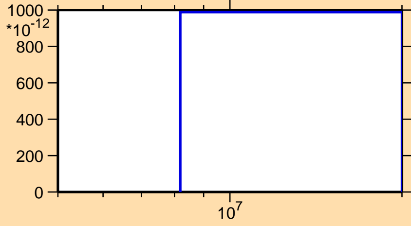
\sigma vs. E for ^{72}\text{Se} (mt 45)
