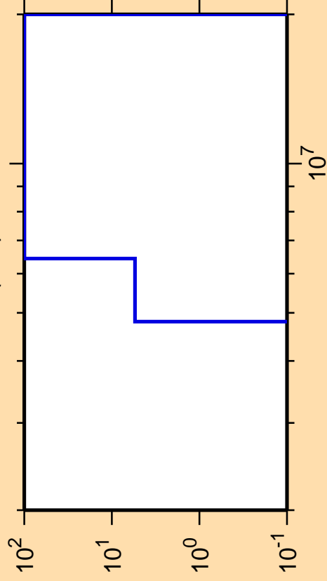
\Delta\sigma/\sigma vs. E for ^{72}\text{Se}(n,d)
