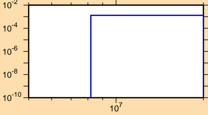
\sigma vs. E for ^{72}\text{Se}(n,p\alpha)
