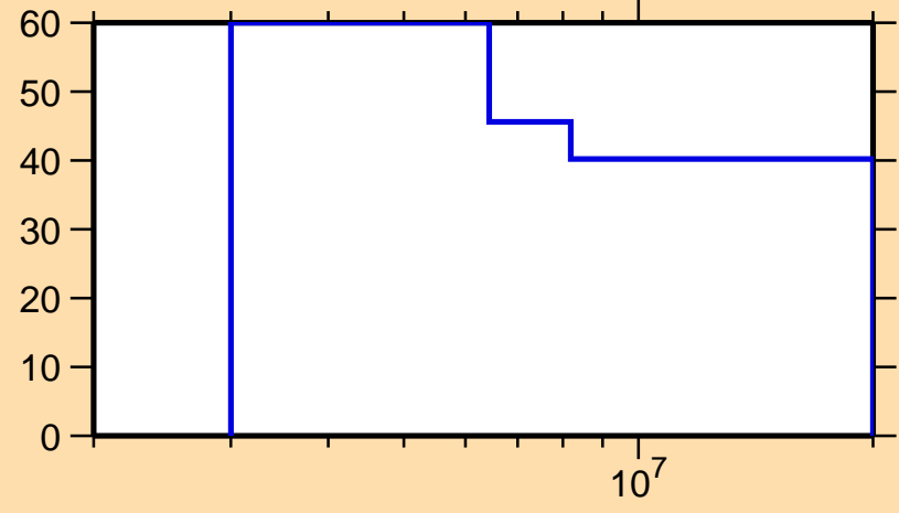
\Delta\sigma/\sigma vs. E for ^{72}\text{Se}(n,n\text{cont.})
