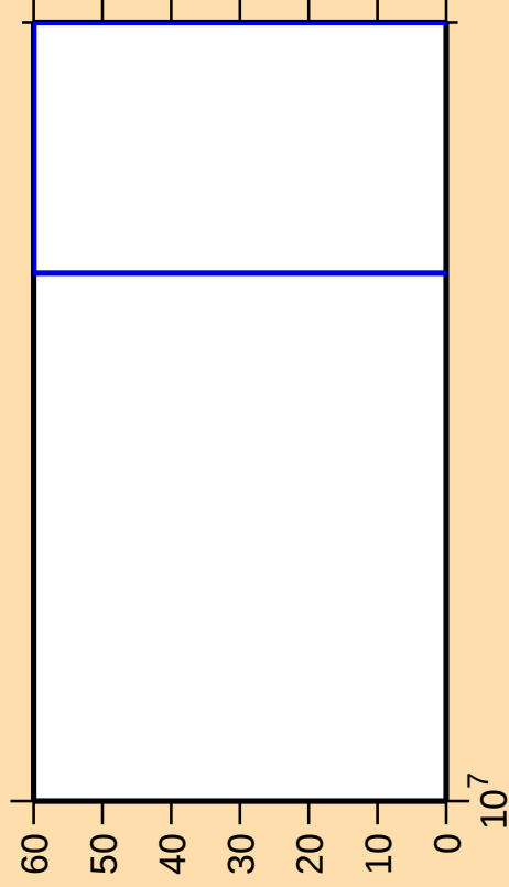
\Delta\sigma/\sigma vs. E for ^{73}\text{Se}(\text{mt } 34)
