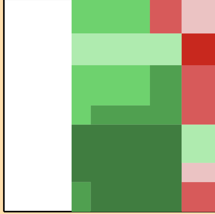
\Delta\sigma/\sigma vs. E for ^{73}\text{Se}(n,2n)
