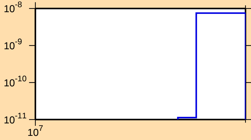
\sigma vs. E for ^{73}\text{Se}(\text{mt 45})
