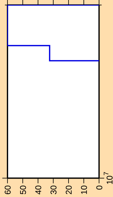
\Delta\sigma/\sigma vs. E for ^{73}\text{Se}(\text{mt 45})
