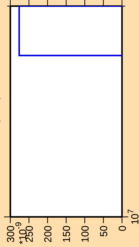
\Delta\sigma/\sigma vs. E for ^{73}\text{Se}(n,\text{nt})
