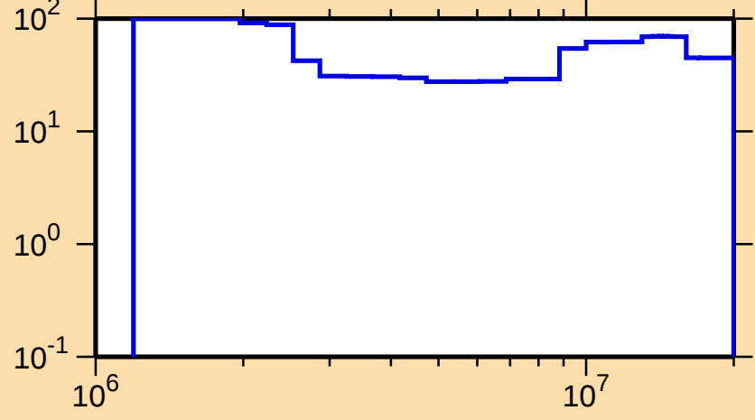
\Delta\sigma/\sigma vs. E for ^{73}\text{Se}(n,n\text{cont.})
